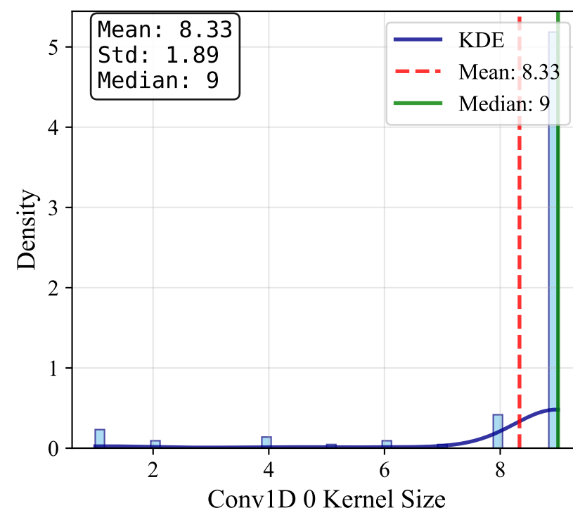
Conv1D 0 Kernel Size
