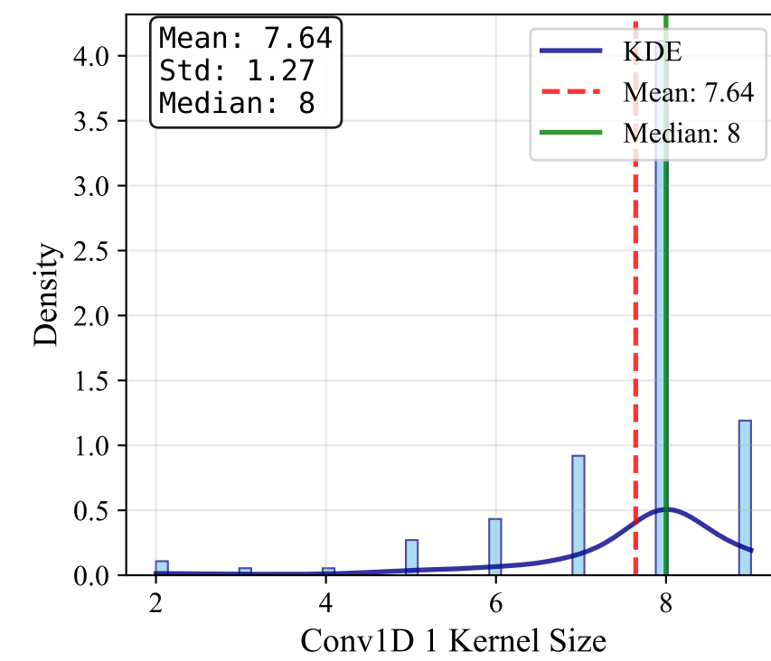
Conv1D 1 Kernel Size
