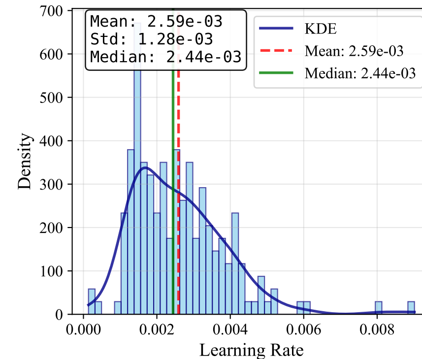
Learning Rate
