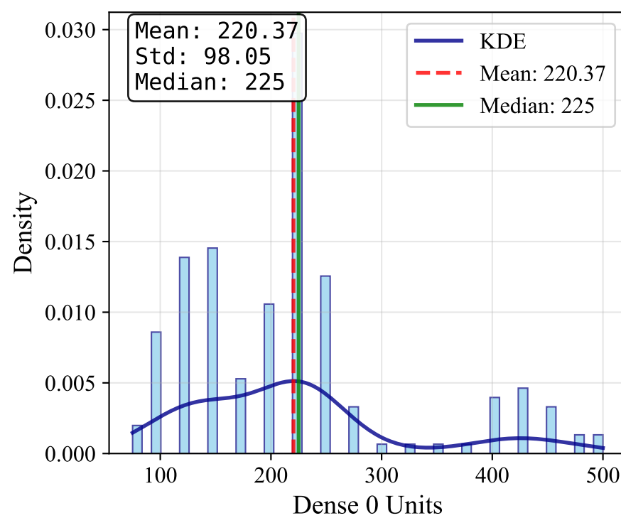
Dense 0 Units
