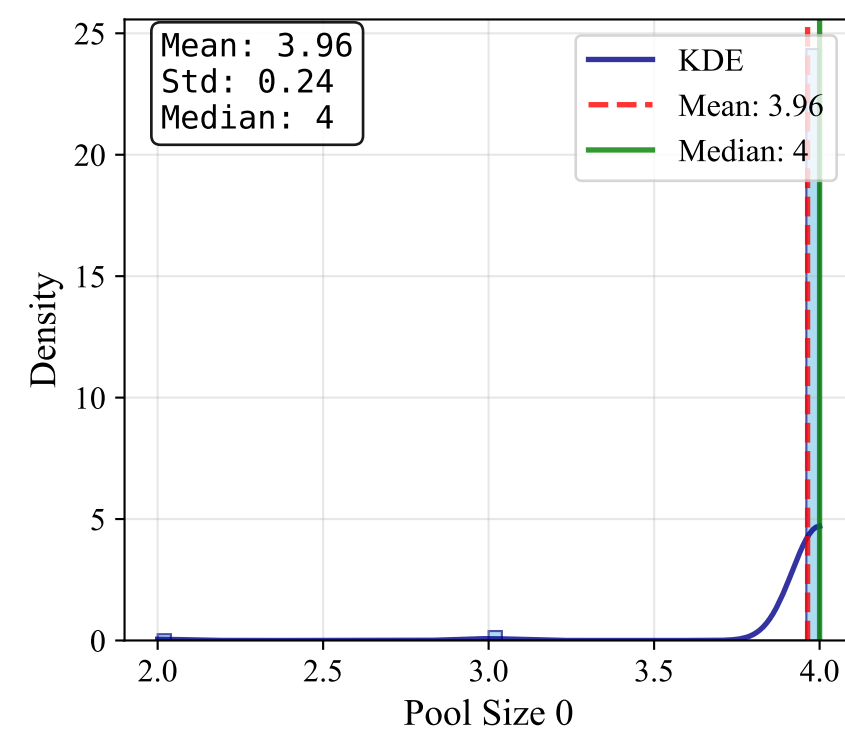
Pool Size 0
