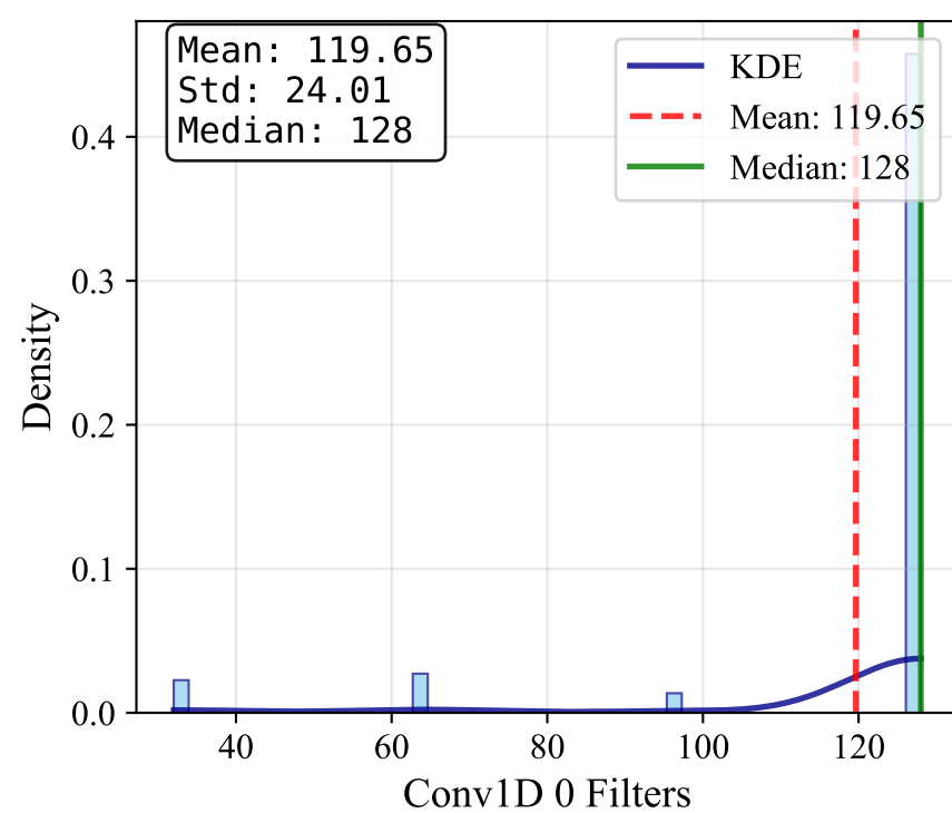
Conv1D 0 Filters
