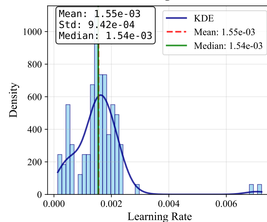
Learning Rate
