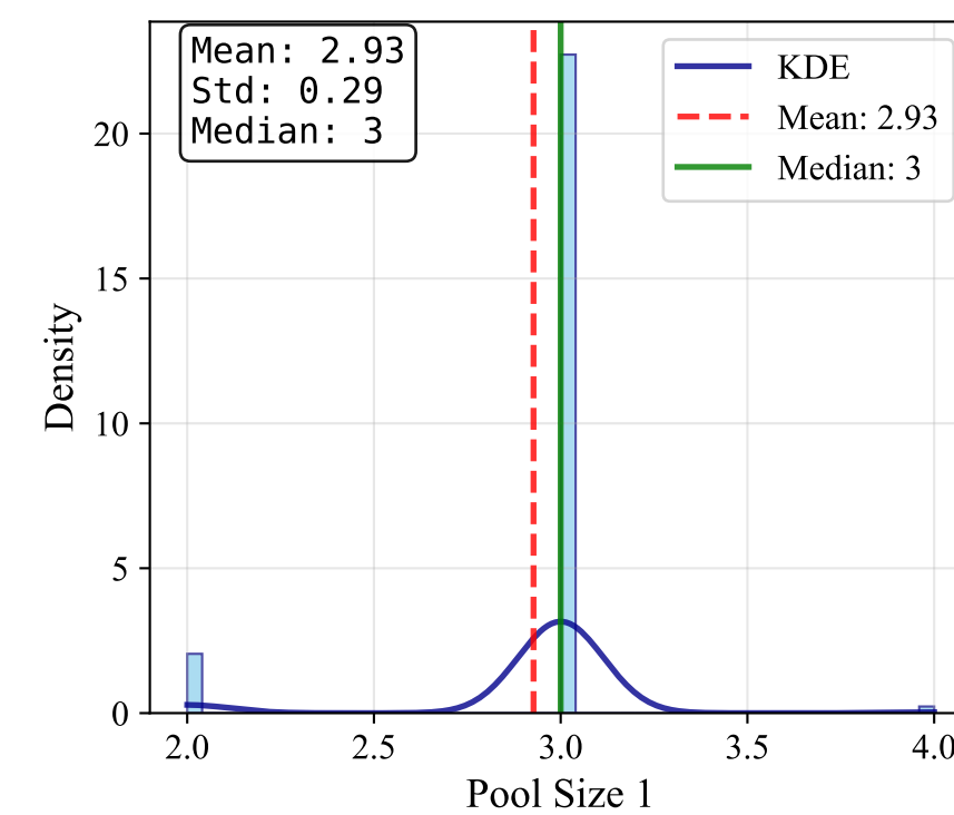
Pool Size 1
