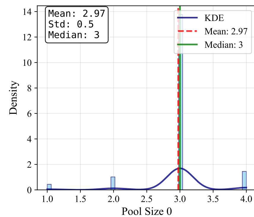
Pool Size 0
