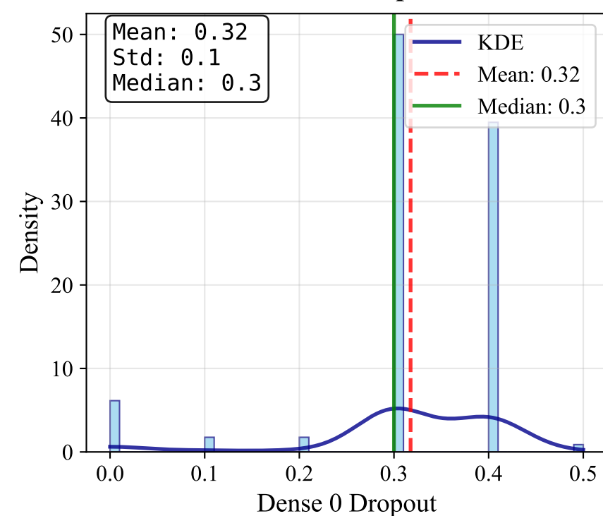
Dense 0 Dropout
