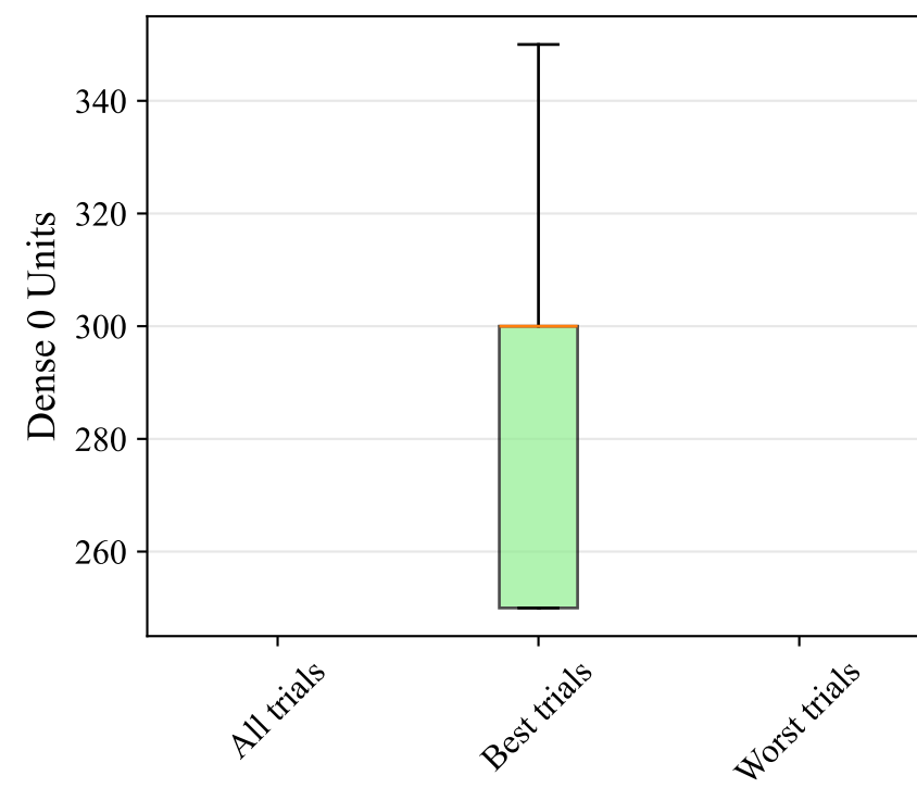
Dense 0 Units
