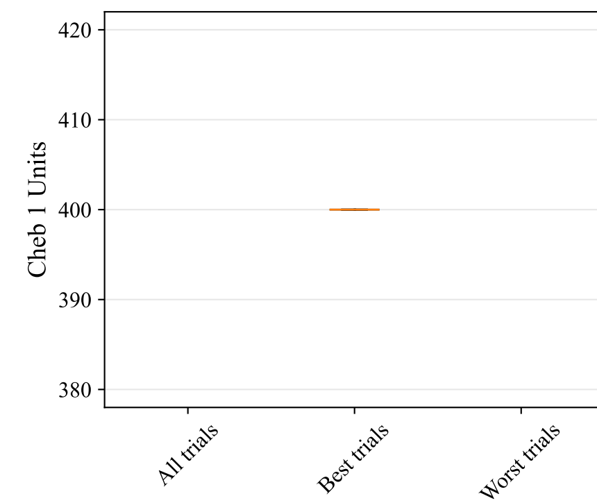
Cheb 1 Units
