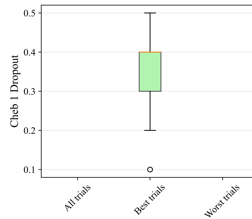
Cheb 1 Dropout
