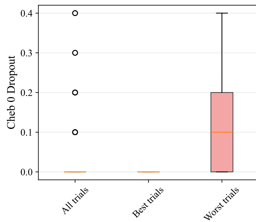
Cheb 0 Dropout
