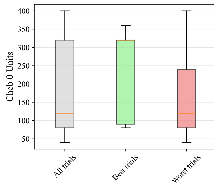
Cheb 0 Units
