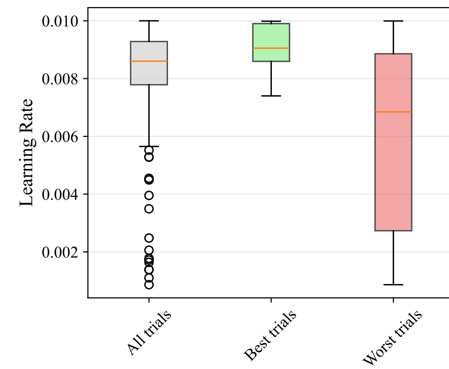
Learning Rate
