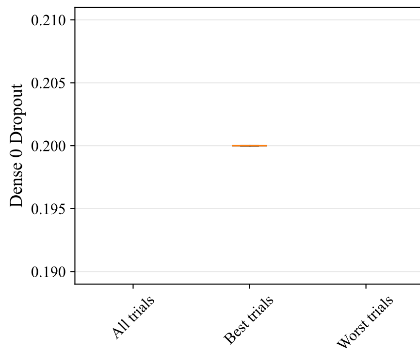
Dense 0 Dropout
