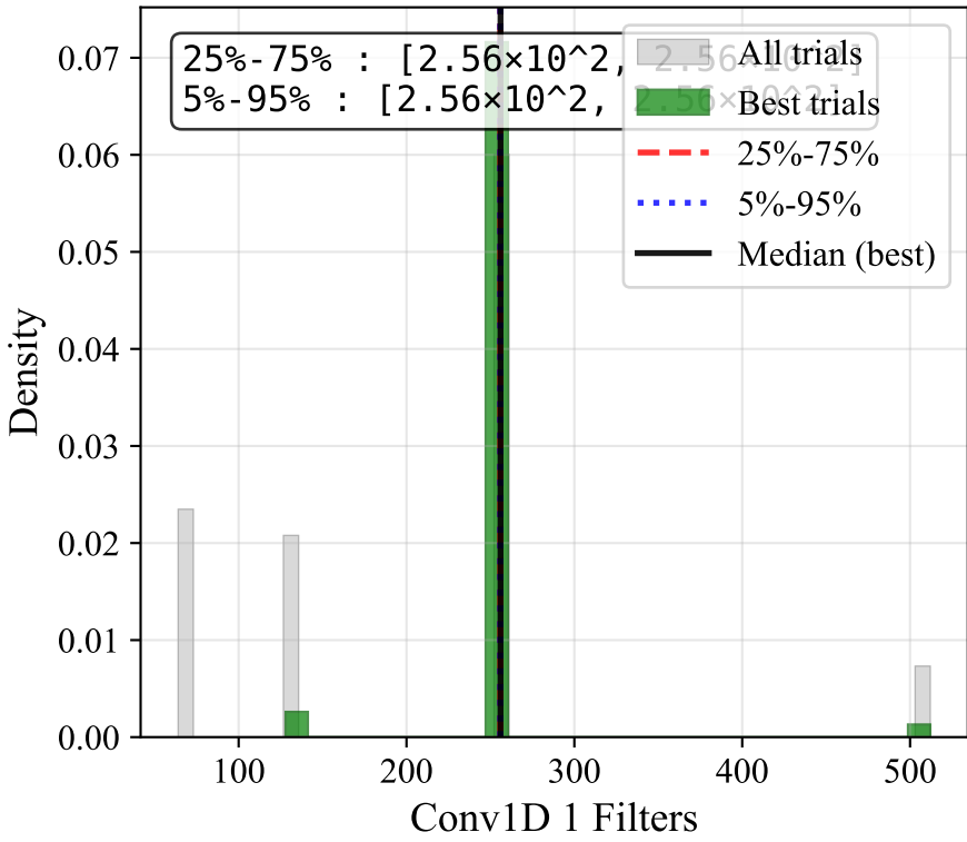
Conv1D 1 Filters
