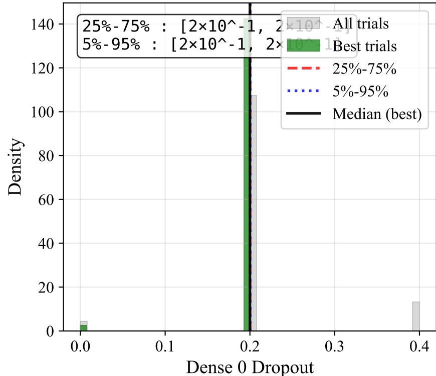
Dense 0 Dropout
