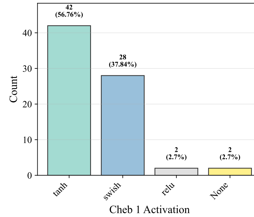
Cheb 1 Activation
