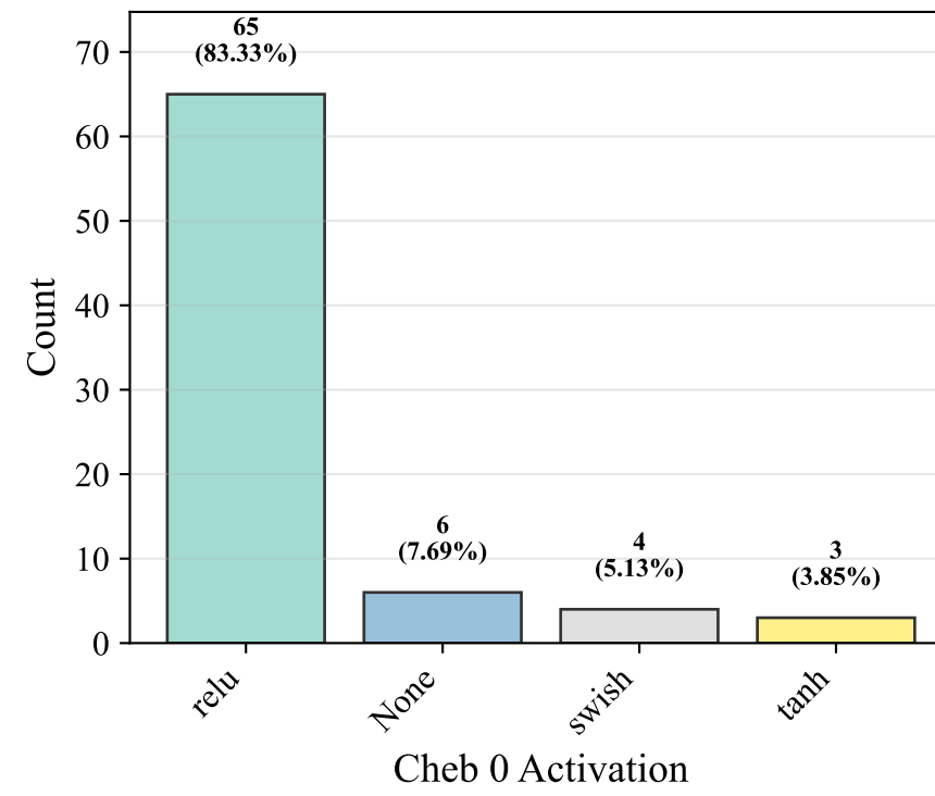
Cheb 0 Activation
