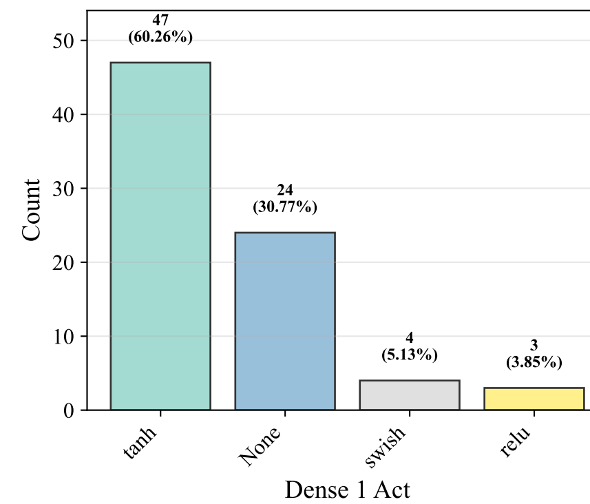
Dense 1 Act
