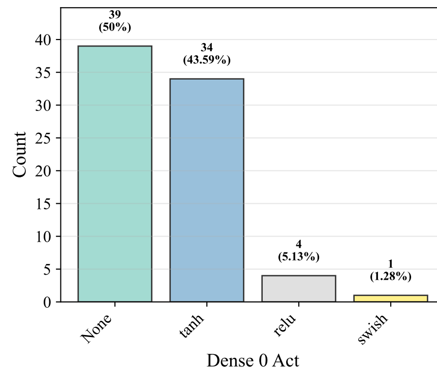
Dense 0 Act
