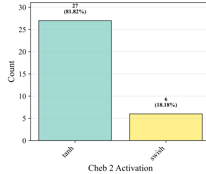
Cheb 2 Activation
