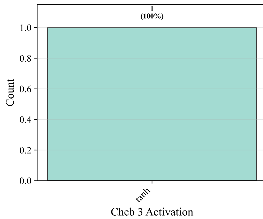
Cheb 3 Activation
