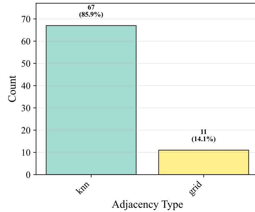
Adjacency Type
