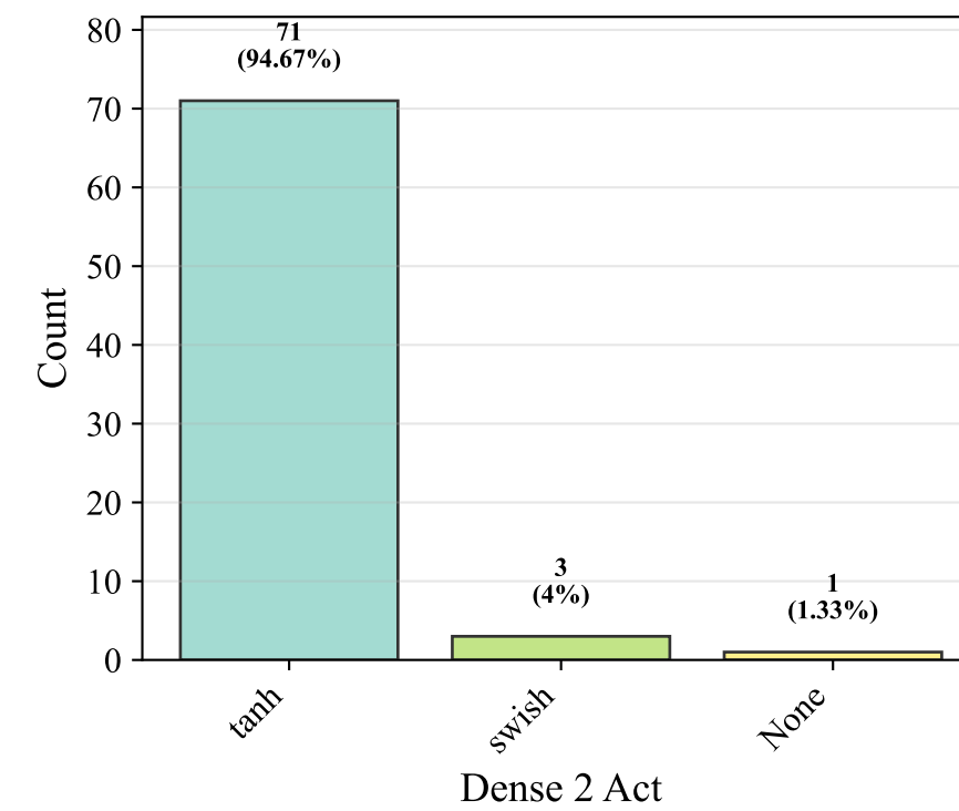
Dense 2 Act
