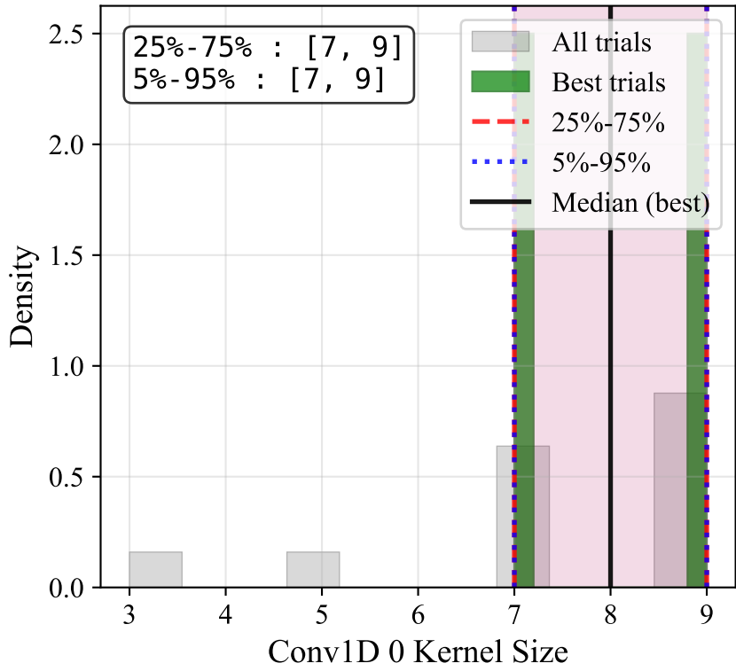
Conv1D 0 Kernel Size
