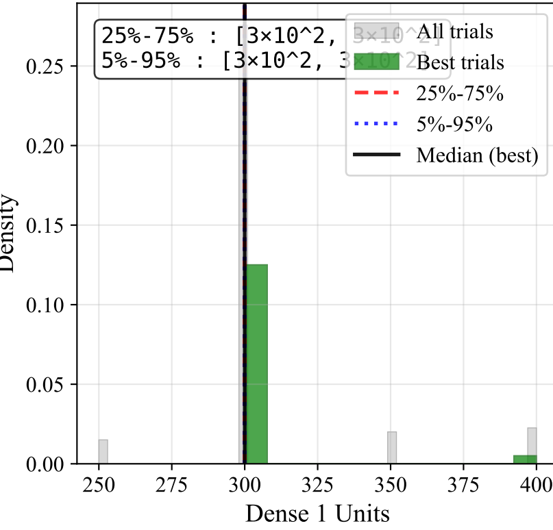
Dense 1 Units
