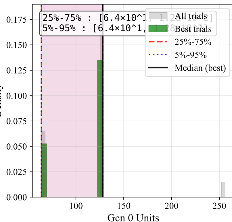
Gen 0 Units
