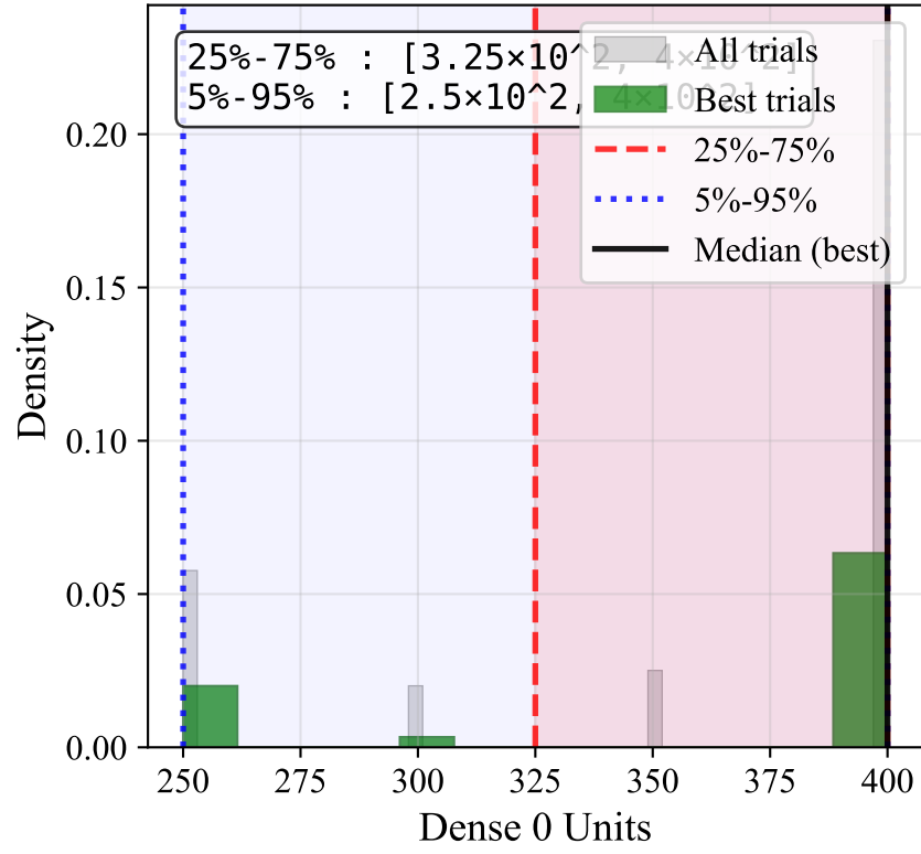
Dense 0 Units
