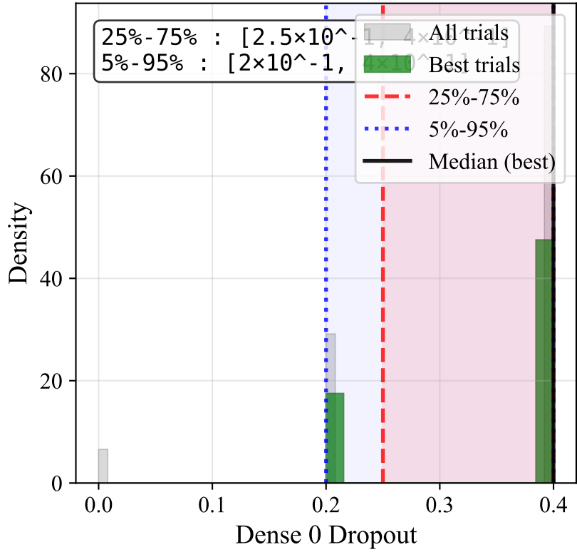
Dense 0 Dropout
