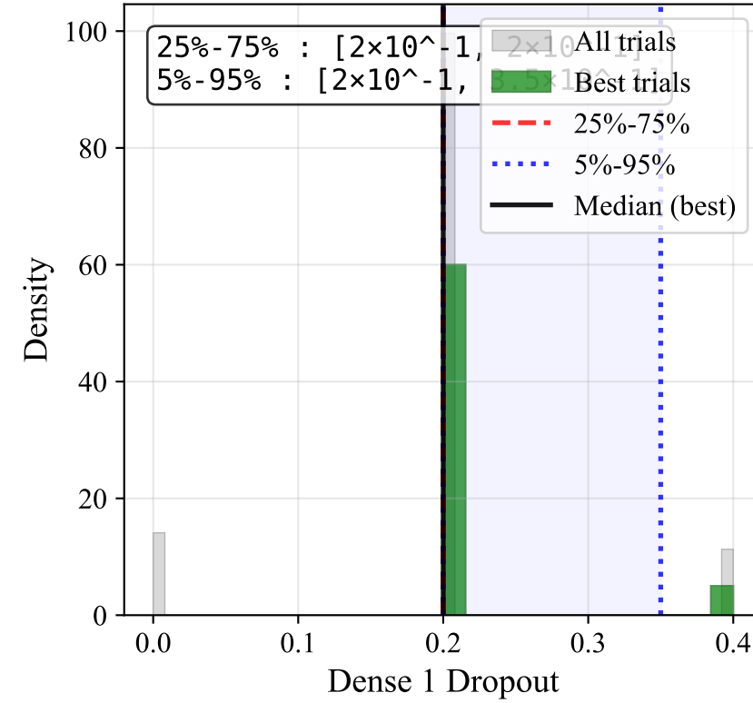
Dense 1 Dropout
