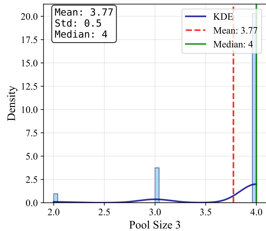
Pool Size 3
