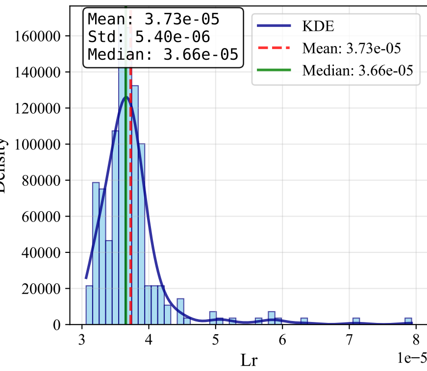
Lr
