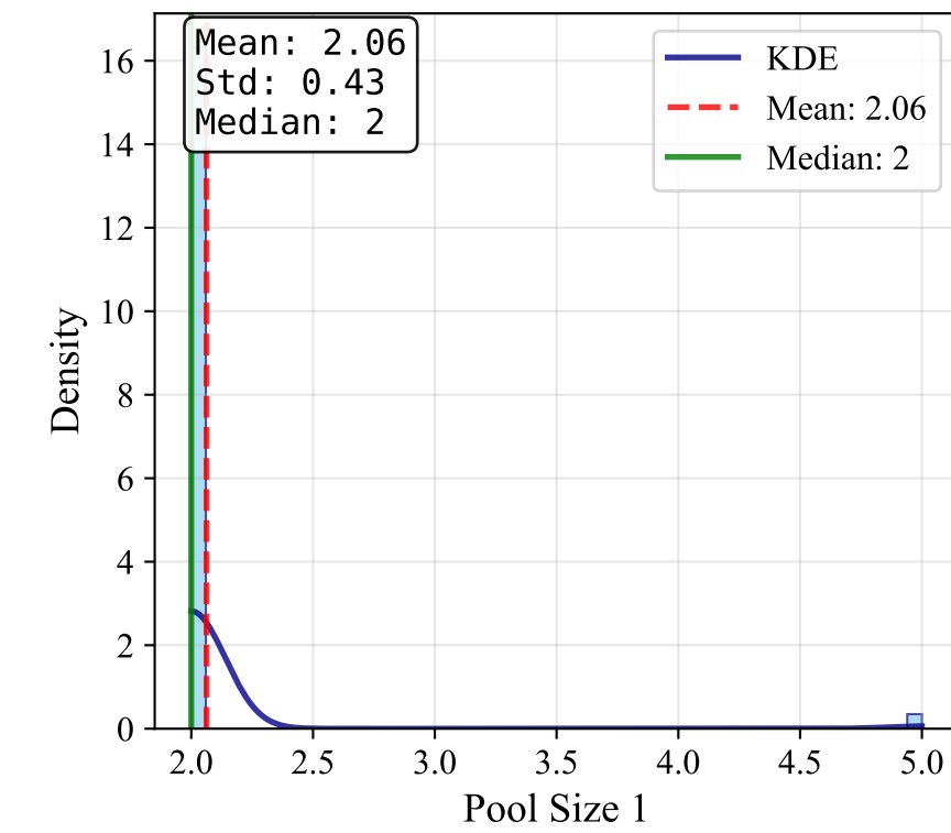
Pool Size 1
