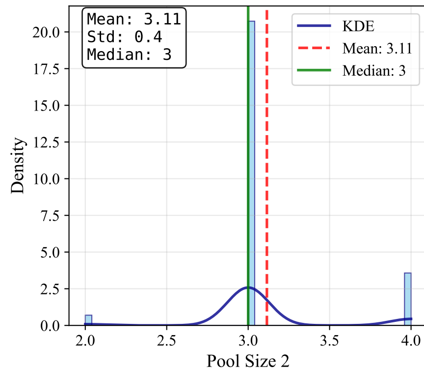
Pool Size 2
