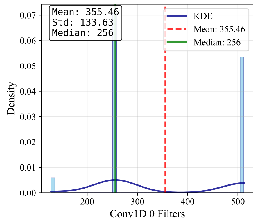
Conv1D 0 Filters
