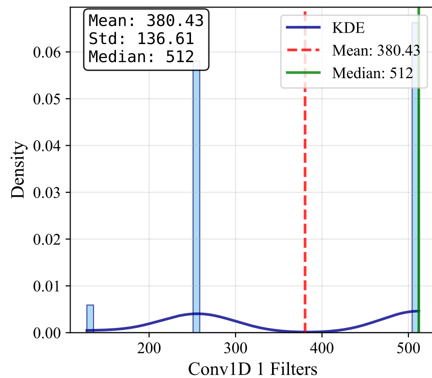
Conv1D 1 Filters
