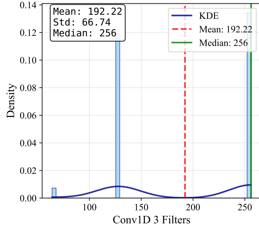
Conv1D 3 Filters
