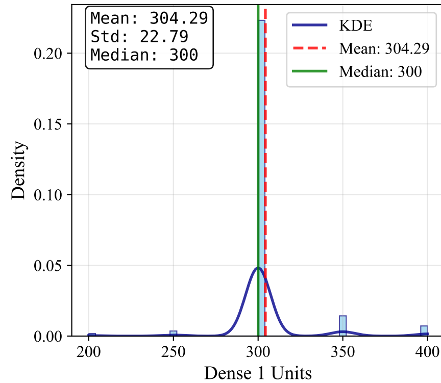
Dense 1 Units
