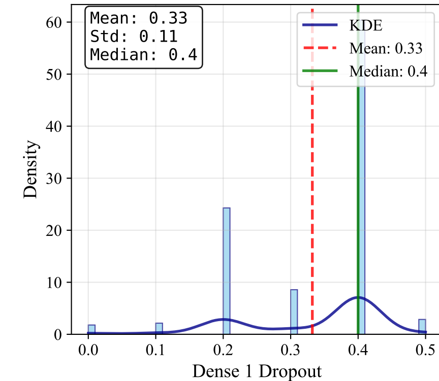
Dense 1 Dropout
