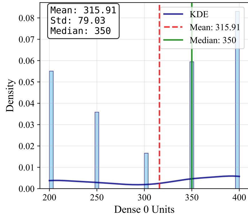
Dense 0 Units
