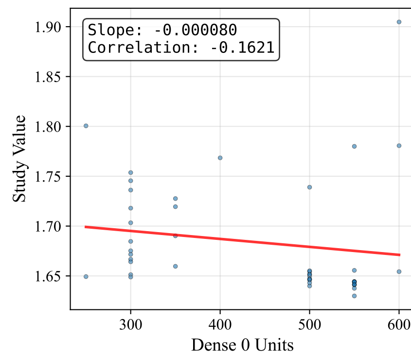
Dense 0 Units
