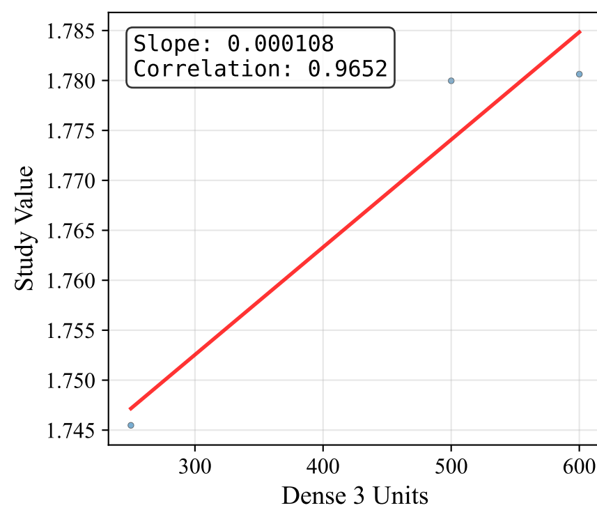
Dense 3 Units
