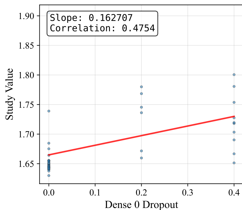
Dense 0 Dropout
