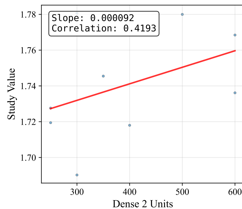
Dense 2 Units
