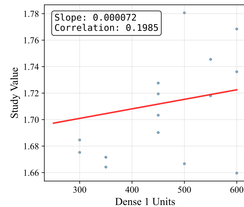
Dense 1 Units
