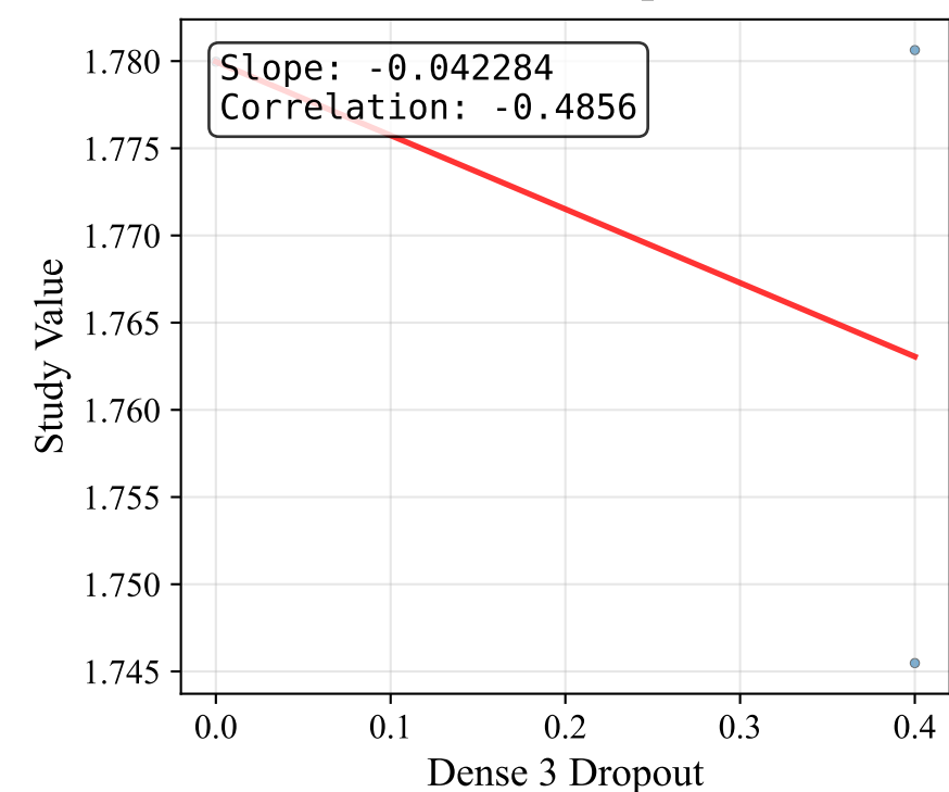
Dense 3 Dropout
