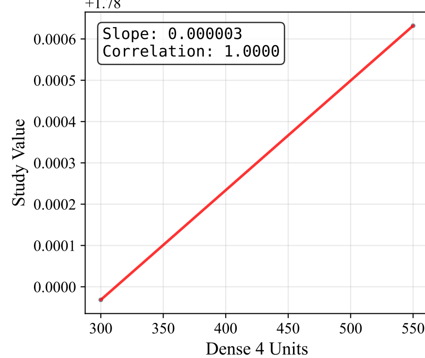
Dense 4 Units
