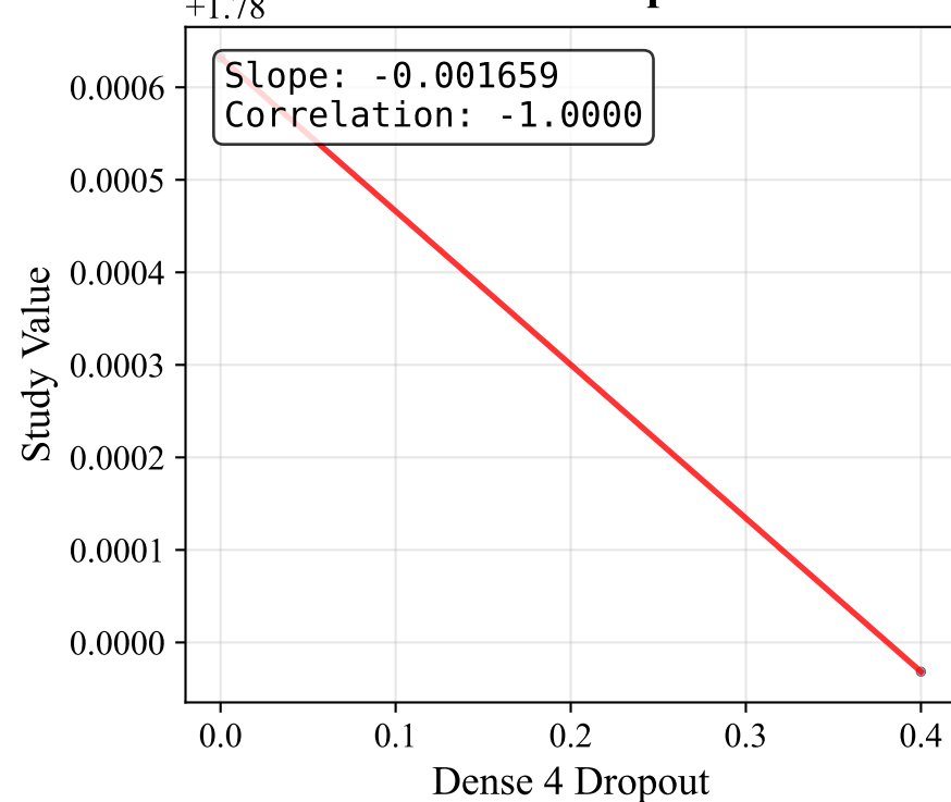
Dense 4 Dropout
