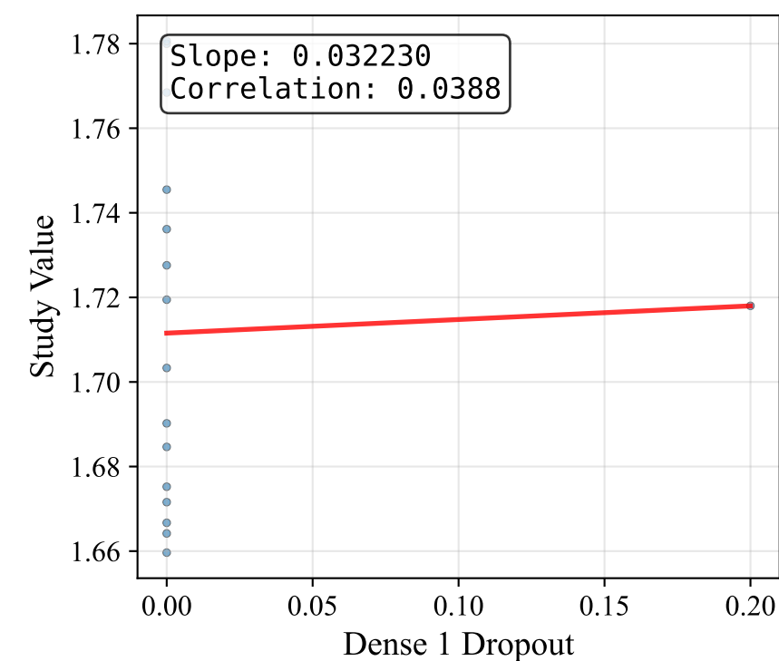
Dense 1 Dropout
