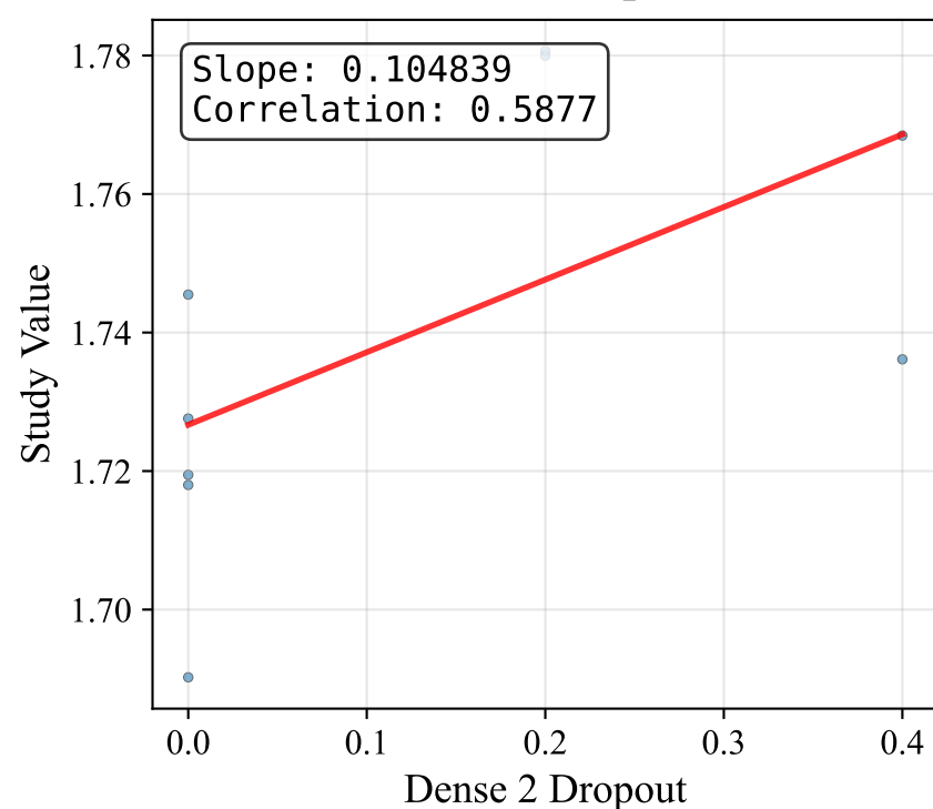
Dense 2 Dropout
