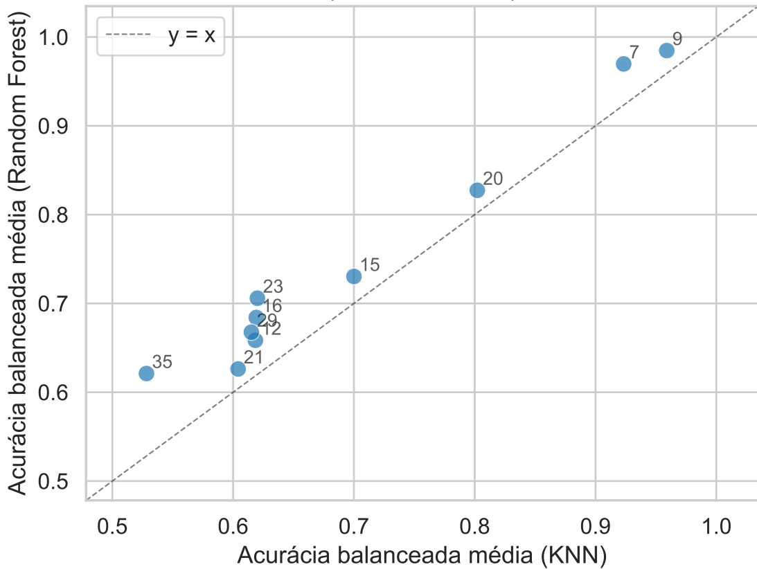
KNN vs Random Forest (Balabit) ( r = 0.99 , n = 10 )
