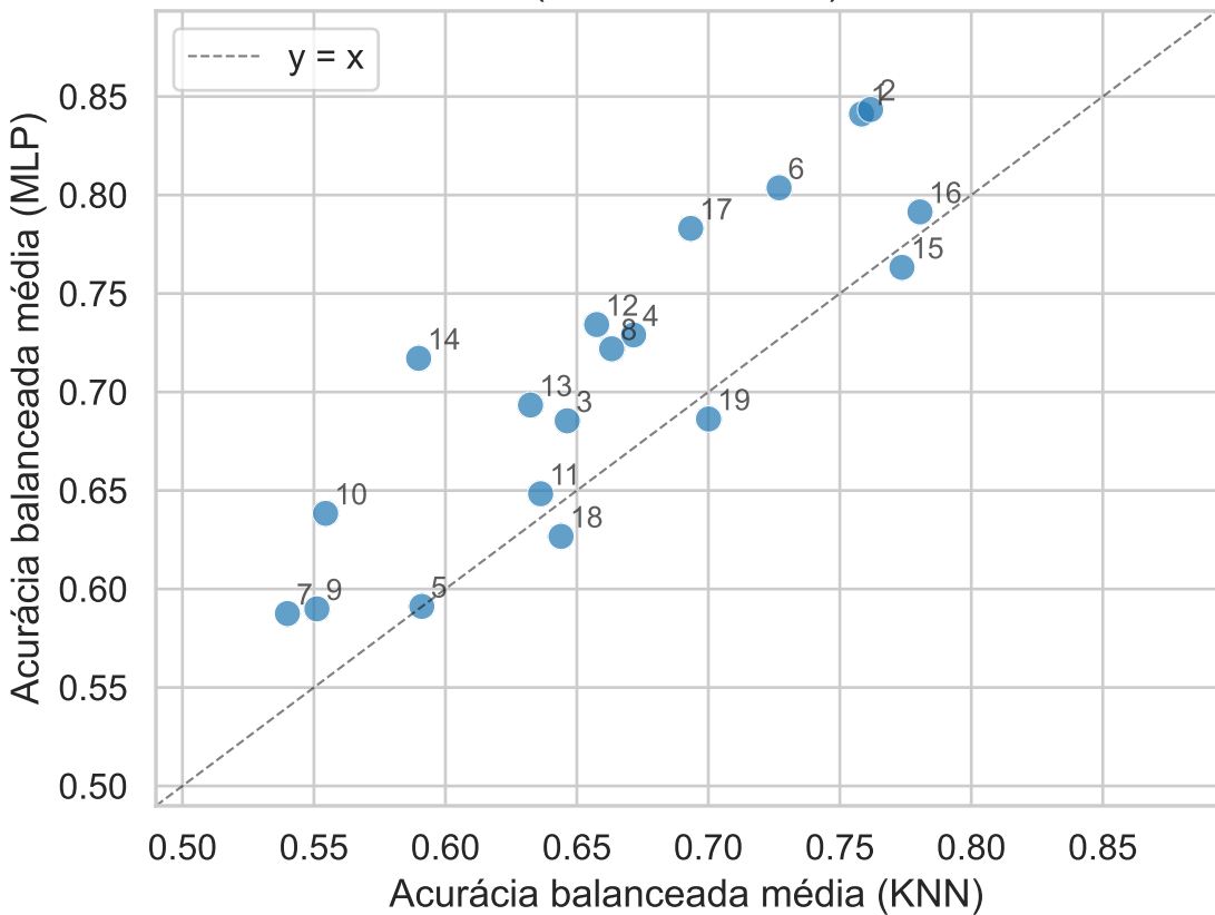
KNN vs MLP (Bogazici) ( r = 0.87 , n = 19 )
