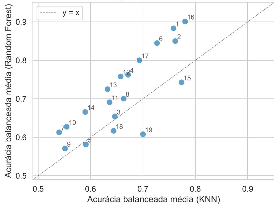
KNN vs Random Forest (Bogazici) ( r = 0.82 , n = 19 )
