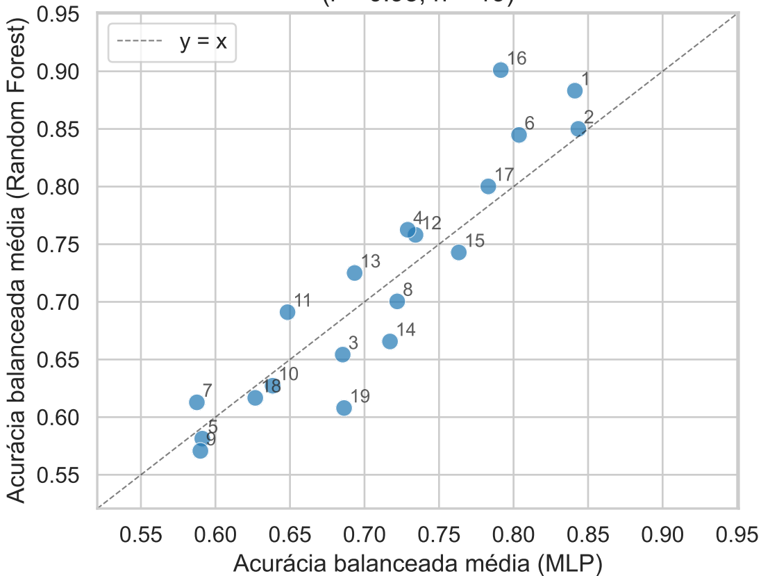
MLP vs Random Forest (Bogazici) ( r = 0.93 , n = 19 )
