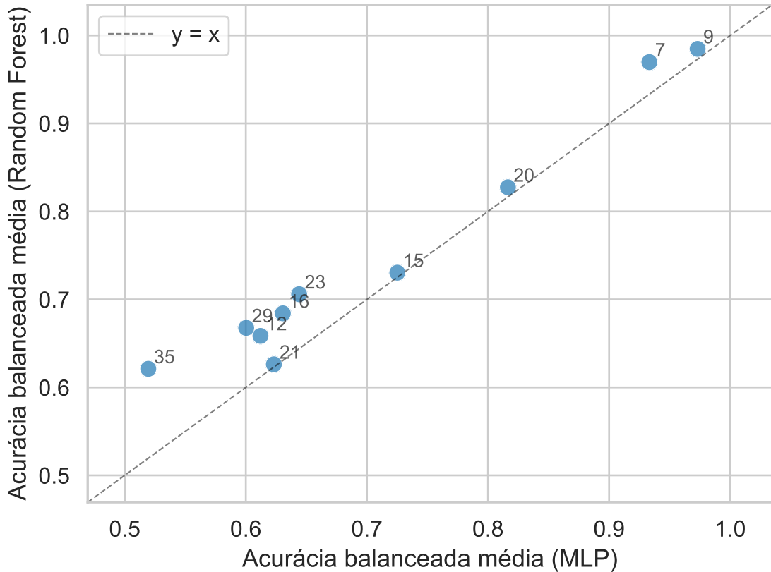
MLP vs Random Forest (Balabit) ( r = 0.98 , n = 10 )
