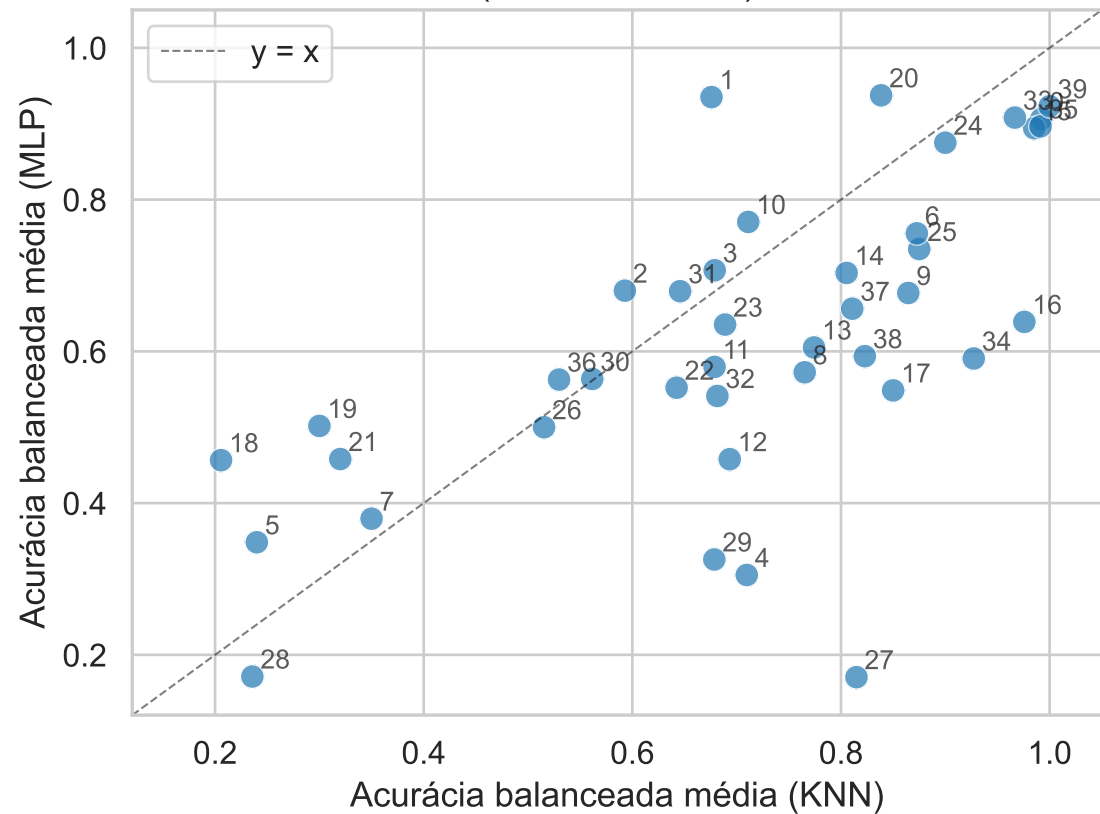
KNN vs MLP (Minecraft) ( r = 0.64 , n = 40 )
