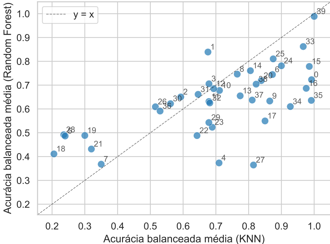
KNN vs Random Forest (Minecraft) ( r = 0.65 , n = 40 )
