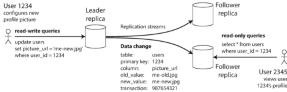
Figure 5-1. Leader-based (master-slave) replication.
