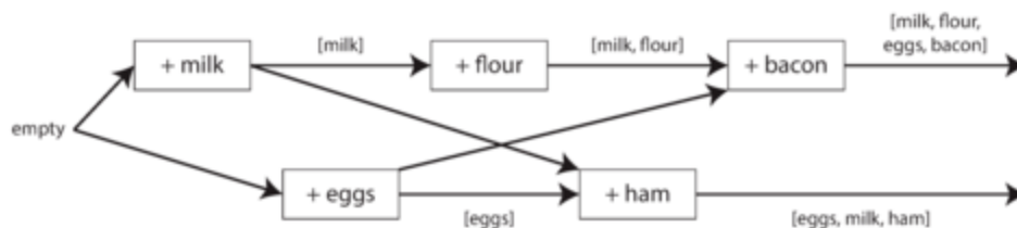
Figure 5-14. Graph of causal dependencies in Figure 5-13.
