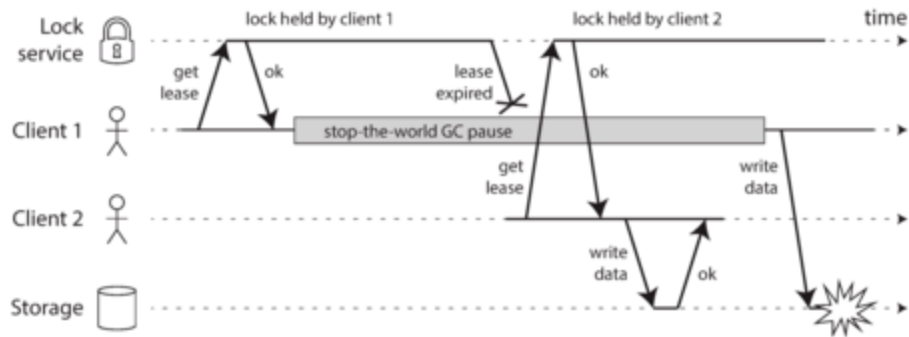
Figure 8-4. Incorrect implementation of a distributed lock: client 1 believes that it still has a valid lease, even though it has expired, and thus corrupts a file in storage.
