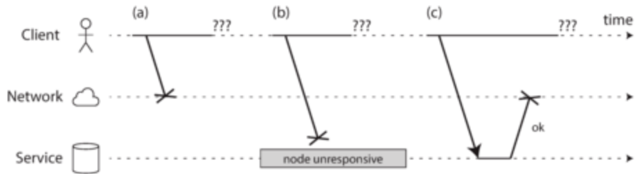
Figure 8-1. If you send a request and don't get a response, it's not possible to distinguish whether (a) the request was lost, (b) the remote node is down, or (c) the response was lost.
