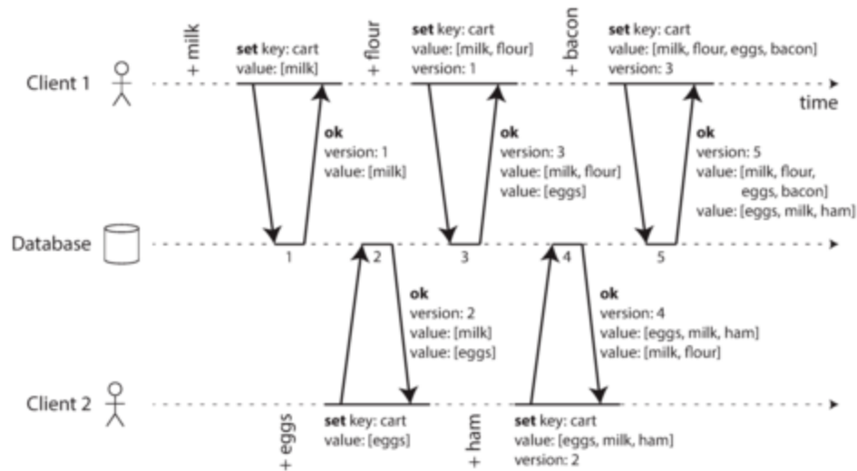
Figure 5-13. Capturing causal dependencies between two clients concurrently editing a shopping cart.
