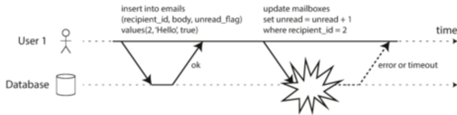
Figure 7-3. Atomicity ensures that if an error occurs any prior writes from that transaction are undone, to avoid an inconsistent state.
