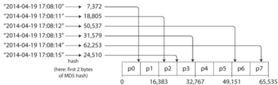
Figure 6-3. Partitioning by hash of key.
