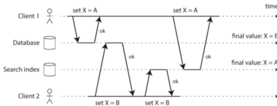
Figure 11-4. In the database, X is first set to A and then to B, while at the search index the writes arrive in the opposite order.
