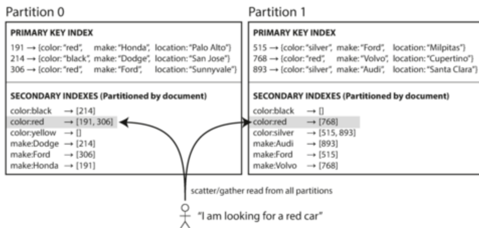
Figure 6-4. Partitioning secondary indexes by document.
