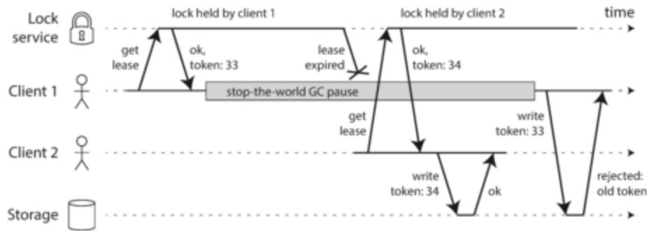
Figure 8-5. Making access to storage safe by allowing writes only in the order of increasing fencing tokens.
