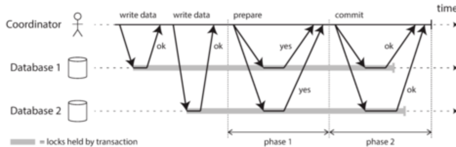
Figure 9-9. A successful execution of two-phase commit (2PC).
