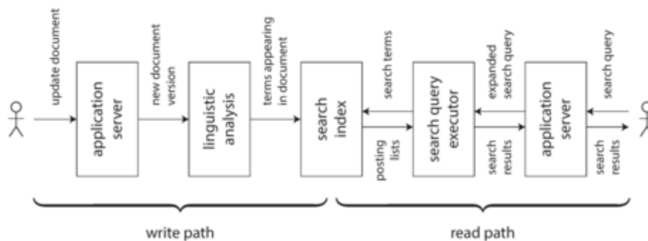
Figure 12-1. In a search index, writes (document updates) meet reads (queries).
