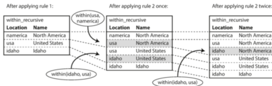
Figure 2-6. Determining that Idaho is in North America, using the Datalog rules from Example 2-11 .
