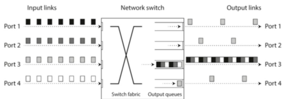
Figure 8-2. If several machines send network traffic to the same destination, its switch queue can fill up. Here, ports 1, 2, and 4 are all trying to send packets to port 3.
