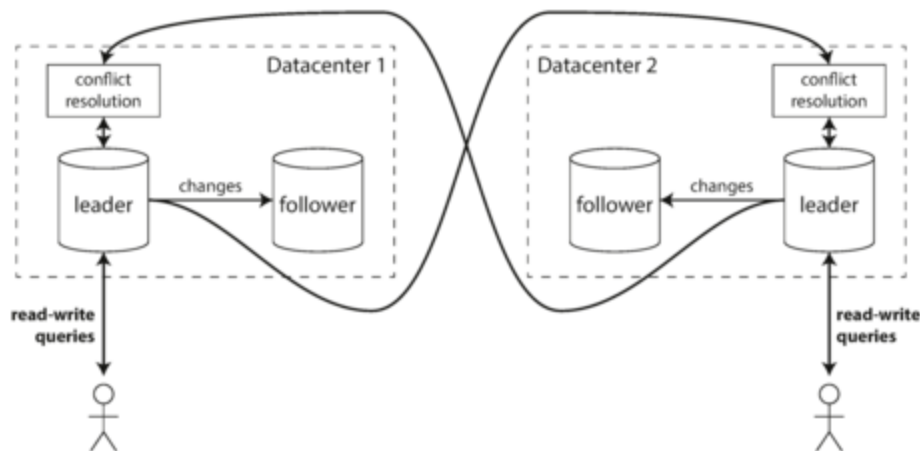
Figure 5-6. Multi-leader replication across multiple datacenters.
