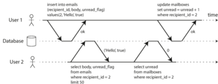
Figure 7-2. Violating isolation: one transaction reads another transaction's uncommitted writes (a "dirty read").
