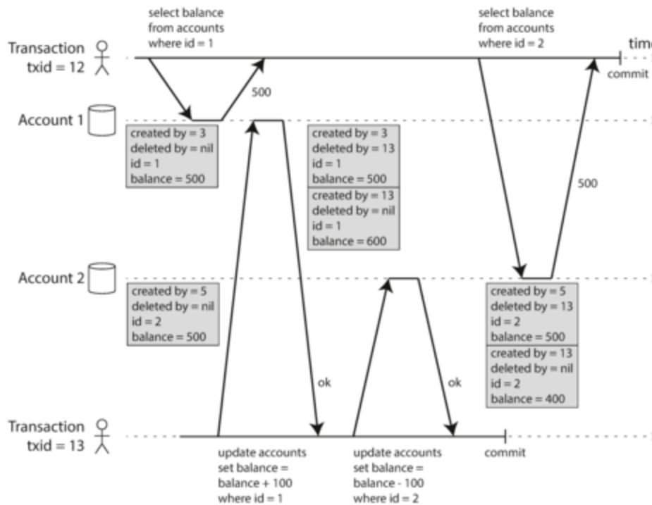
Figure 7-7. Implementing snapshot isolation using multi-version objects.
