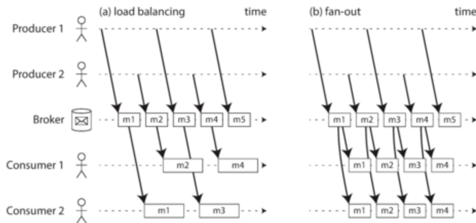
Figure 11-1. (a) Load balancing: sharing the work of consuming a topic among consumers; (b) fan-out: delivering each message to multiple consumers.
