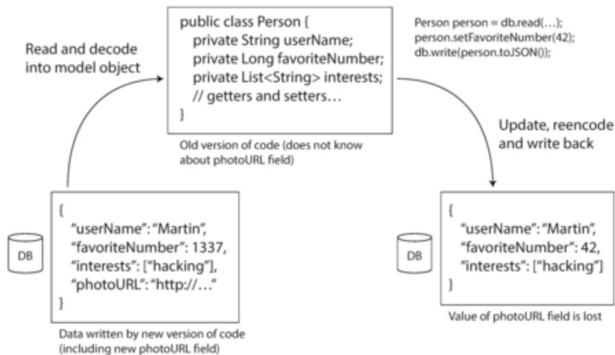
Figure 4-7. When an older version of the application updates data previously written by a newer version of the application, data may be lost if you're not careful.
