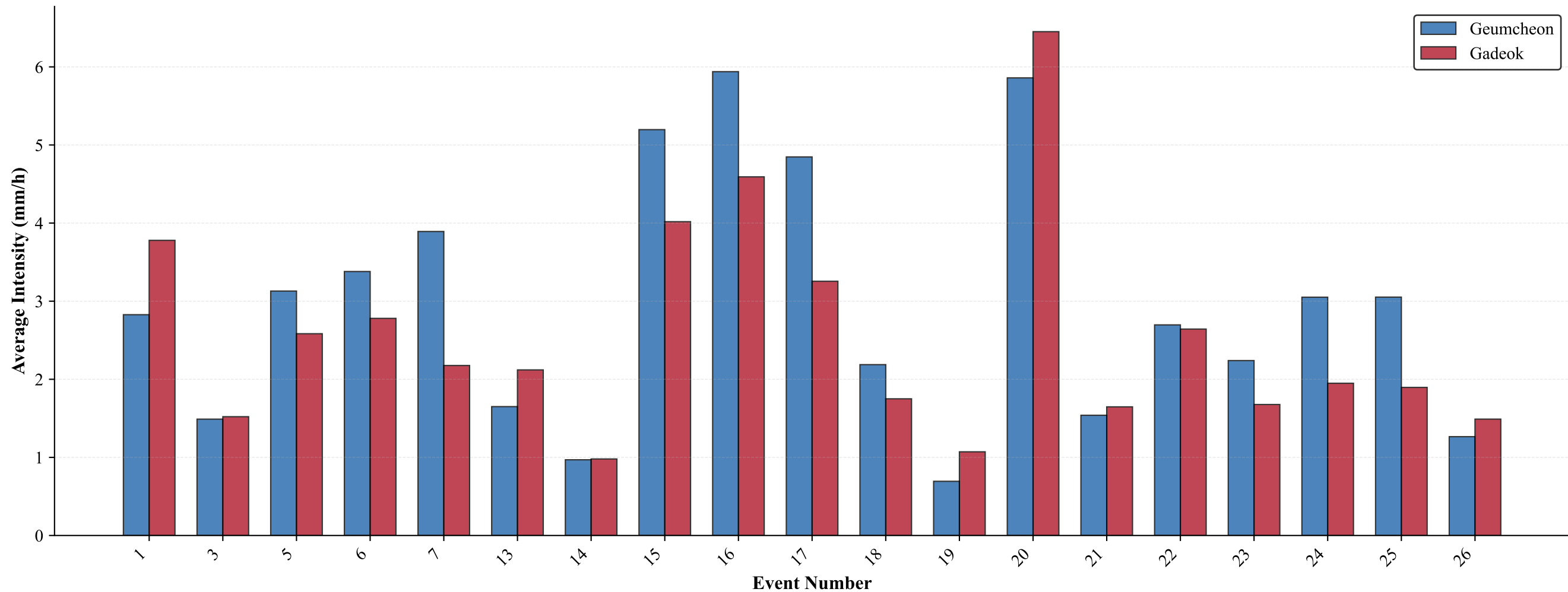
Average Rainfall Intensity (Simultaneous Rainfall, n=19)
