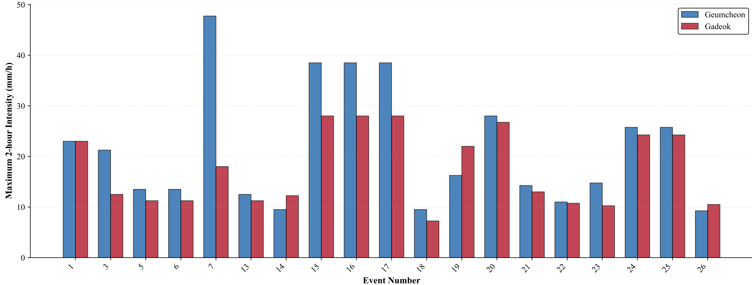
Maximum 2-hour Rainfall Intensity (Simultaneous Rainfall, n=19)
