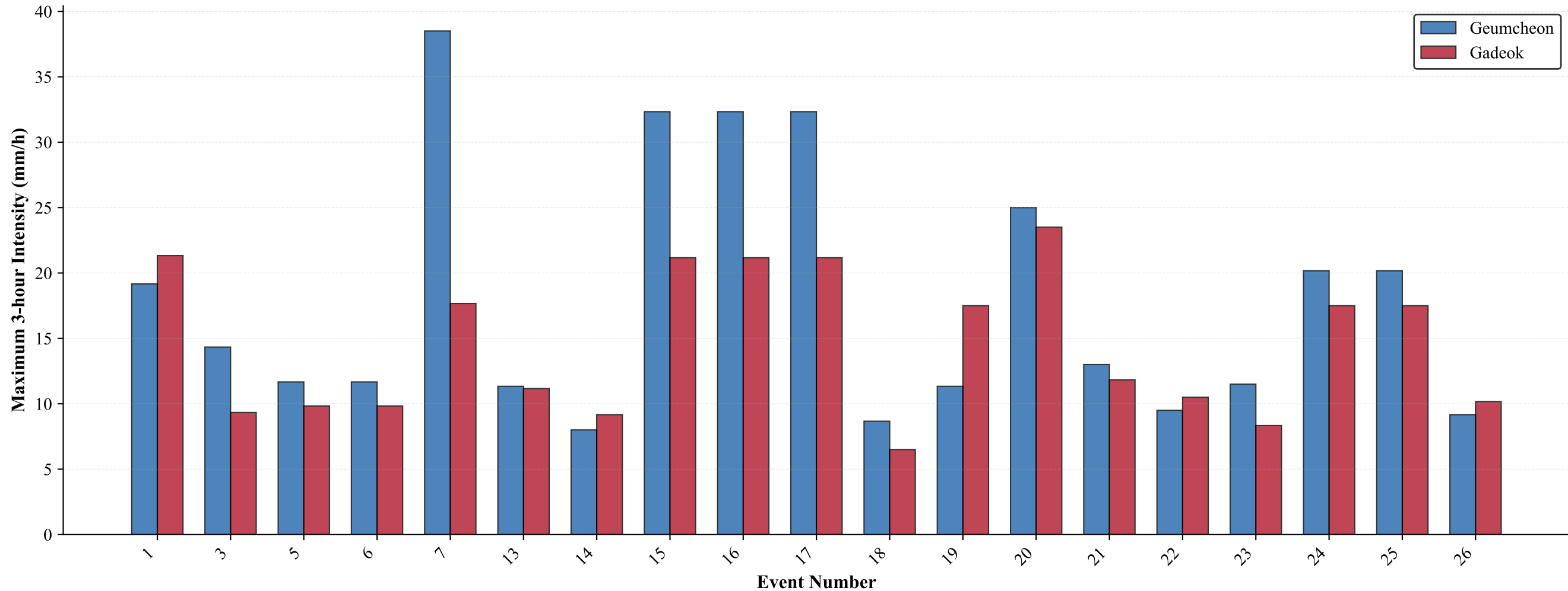
Maximum 3-hour Rainfall Intensity (Simultaneous Rainfall, n=19)
