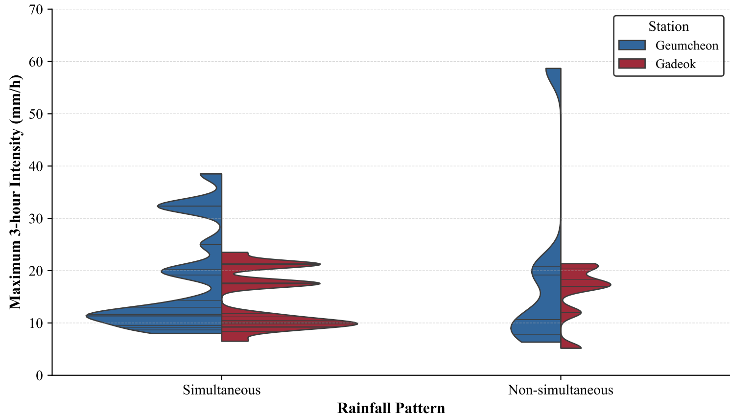
Distribution of Maximum 3-hour Rainfall Intensity
