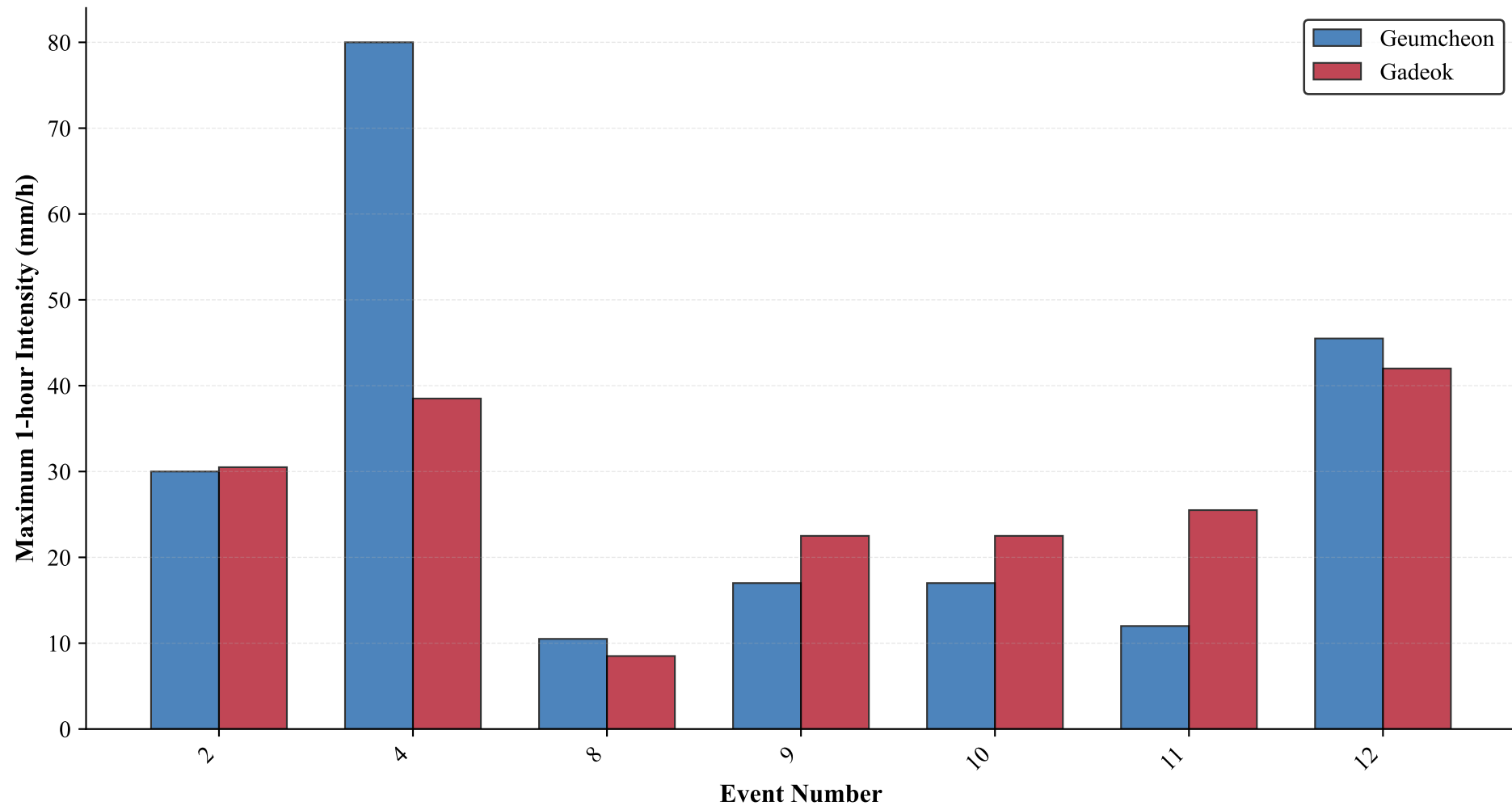
Maximum 1-hour Rainfall Intensity (Non-simultaneous Rainfall, n=7)
