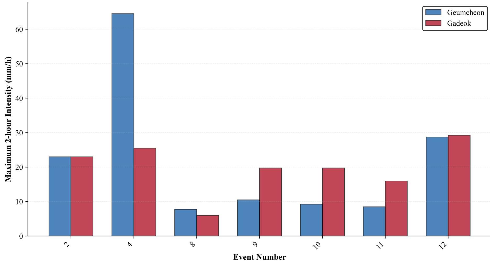
Maximum 2-hour Rainfall Intensity (Non-simultaneous Rainfall, n=7)
