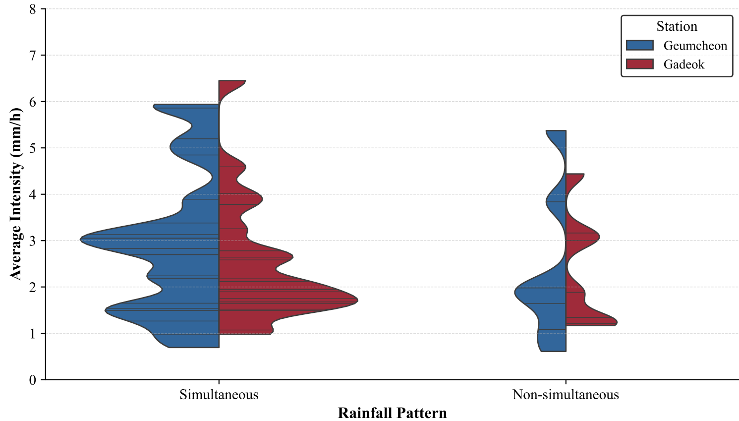
Distribution of Average Rainfall Intensity
