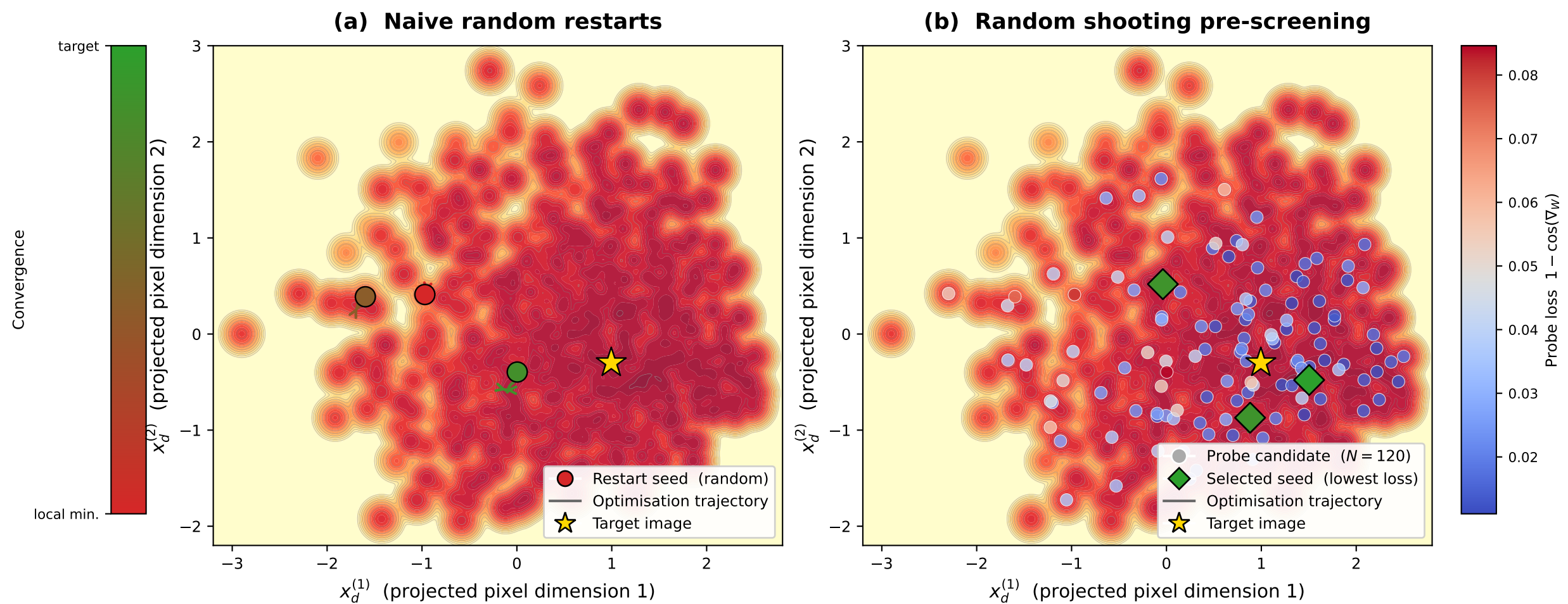
Figure: 2D PCA projection of grayscale LFW faces. Colour shows the true gradient-matching loss 1 - \cos(\nabla_w \mathcal{L}(x_d), \nabla_w \mathcal{L}(x)) (random LeNet), evaluated by inverting the PCA projection at each point. (a) Naive restarts land in high-loss basins. (b) Random shooting evaluates N probes, selects lowest-loss seeds (diamonds), and steers restarts toward the target image — though not all converge (see convergence scale).
