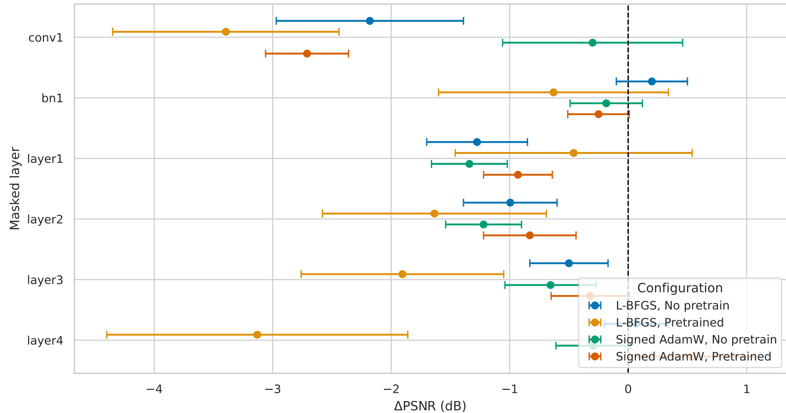
ResNet18 Ablation Study PSNR Difference (Masked – Baseline)
