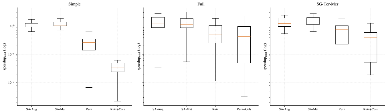
FIGURE 2 At 1% MIPGap, the Gurobi total-time speedup distributions place the structure-aware variants mostly above parity, while Ruiz-type baselines are more dispersed. The axis is the logged total-time speedup of the main campaign ( equation (46) , q = \text{total} ). Its preprocessing component has whole-second resolution: the Ruiz overhead is visible and pulls those medians well below the solver-time and deterministic-effort parity of table 7 and the \rho_{\kappa}^{\text{solver}} scatter, whereas the subsecond structure-aware overhead is rounded to zero ( section 5.5 ). The figure should therefore not be read as a precise preprocessing-plus-solver comparison for the structure-aware variants; those come from the instrumented control batches of section 6.7 . Values above the parity line indicate acceleration relative to the unscaled model. In all box plots, boxes span the interquartile range (IQR) and whiskers extend to the most extreme observation within 1.5 \times \text{IQR} ; outliers are omitted, since tail behavior is captured by PAR10 and the performance profiles.
