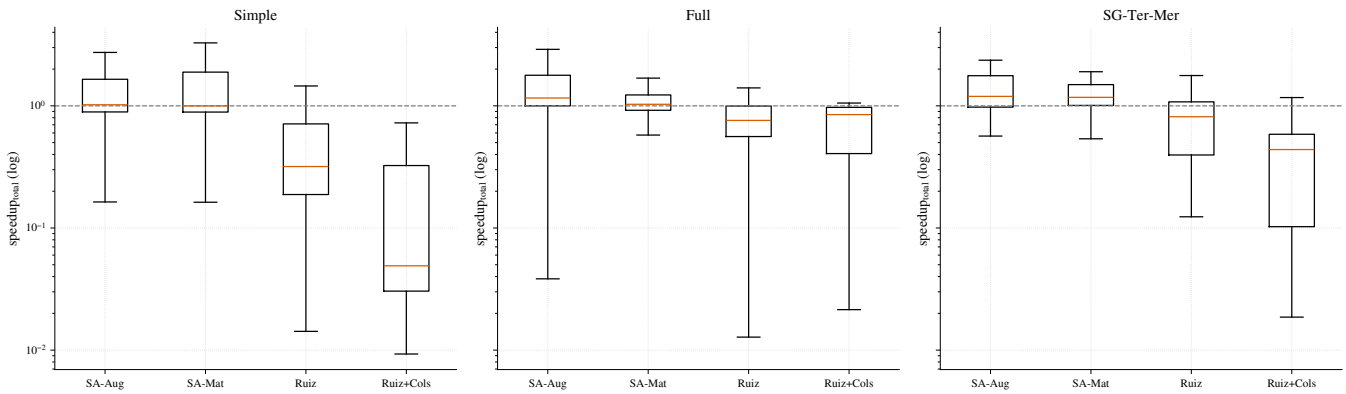
FIGURE 5 At 0.1% MIPGap, the Gurobi speedup distributions preserve the same qualitative pattern observed at the looser tolerance. Values above one indicate faster runs than the unscaled formulation.
