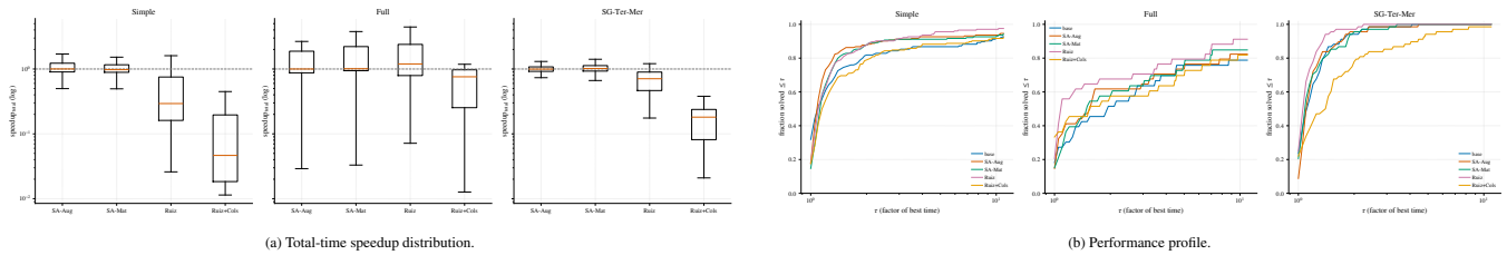
FIGURE 9 At 0.1% MIPGap, the CPLEX visual evidence remains mixed under the stricter tolerance, supporting a solver-dependent interpretation.
