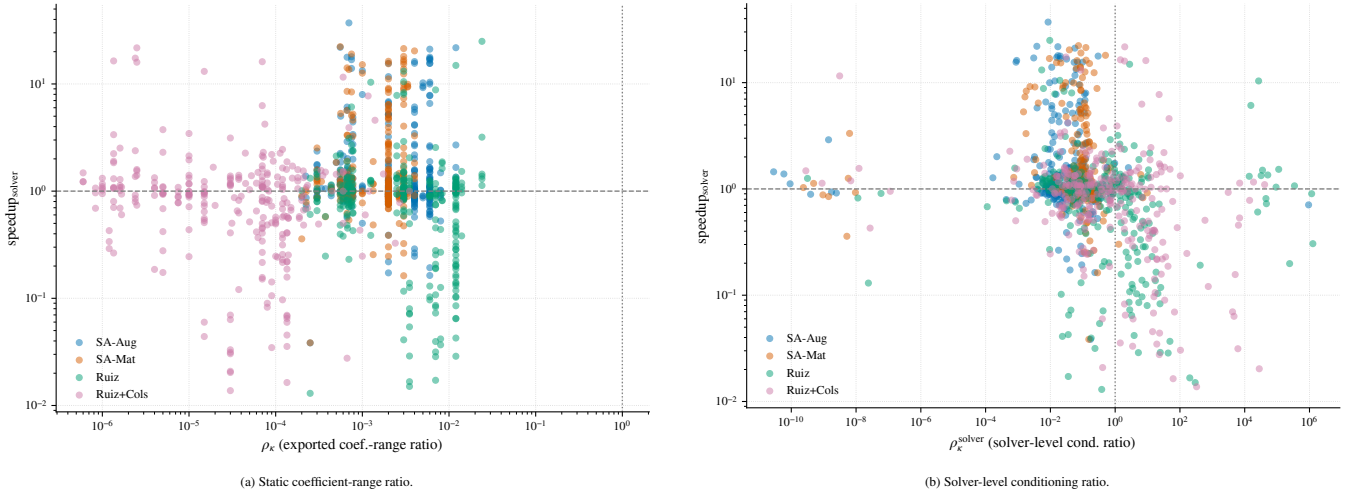
FIGURE 6 At 0.1% MIPGap, the stricter Gurobi runs again separate static coefficient compression from solver-facing numerical behavior. The solver-level diagnostic remains more informative than the exported coefficient-range ratio.
