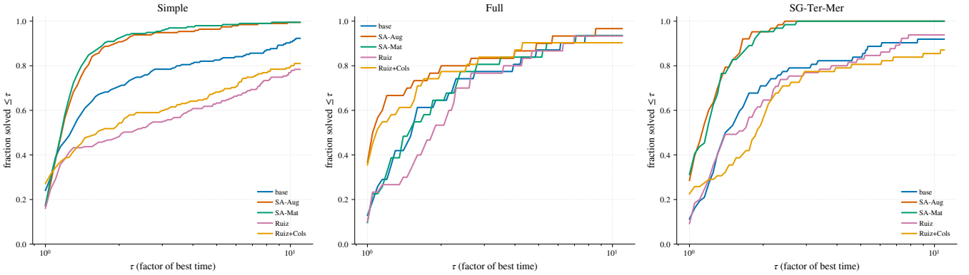
FIGURE 7 At 0.1% MIPGap, the Dolan–Moré profiles test whether the Gurobi speedups persist across the heterogeneous instance pool rather than only in averages.
