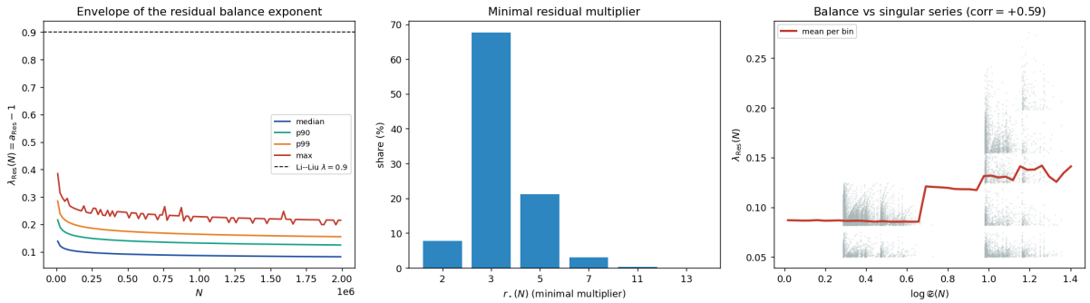
Figure 6: Left: percentile envelope of \lambda_{\text{Res}} = a_{\text{Res}} - 1 versus N , far below the Li–Liu line 0.9. Centre: the minimal multiplier r_\star ( r = 3 dominates). Right: \lambda_{\text{Res}} rises with the Goldbach singular series \mathfrak{S}(N) (positive correlation).
