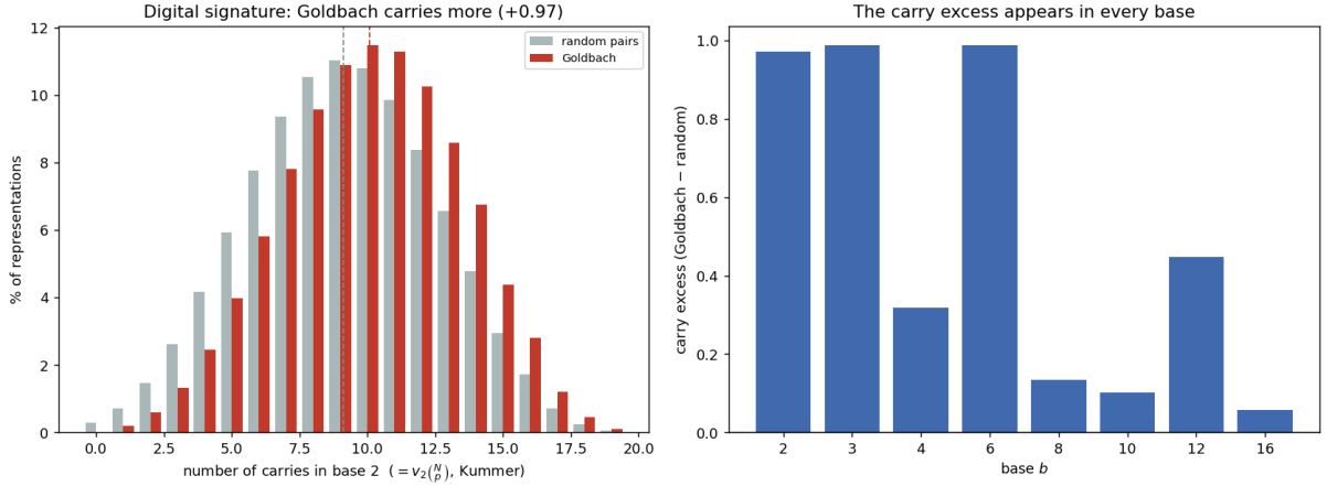
Figure 8: Carry geometry. Left: the distribution of binary carries v_2(\binom{N}{p}) for Goldbach representations (red) versus random pairs (grey)—Goldbach is shifted to more carries (+0.97). Right: the carry excess is positive in every base.
