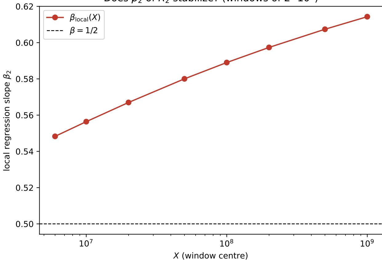
Does \beta_2 of R_2 stabilize? (windows of 2 \cdot 10^6 )
