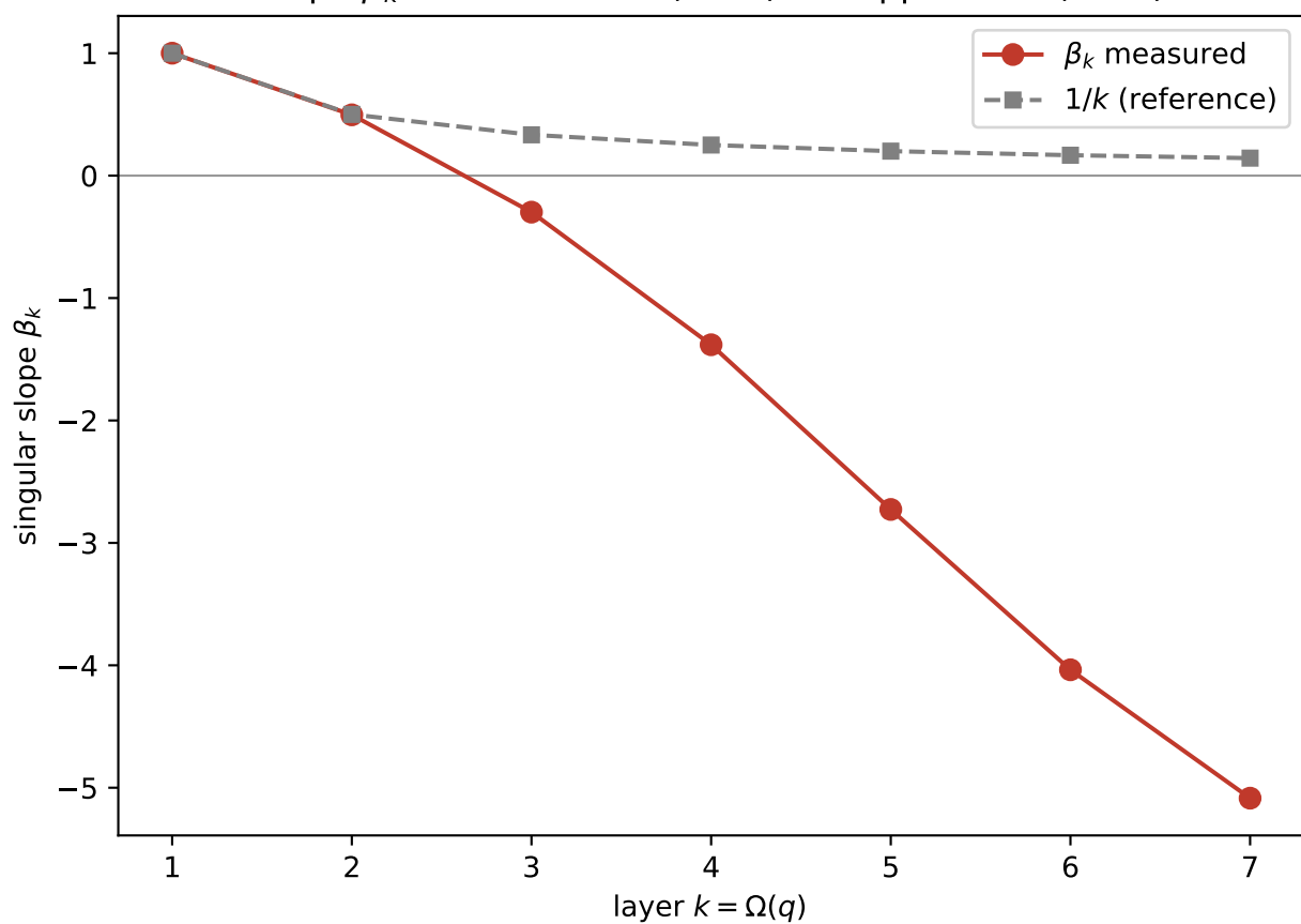
Slope \beta_k : enhancement ( k \leq 2 ) vs suppression ( k \geq 3 )
