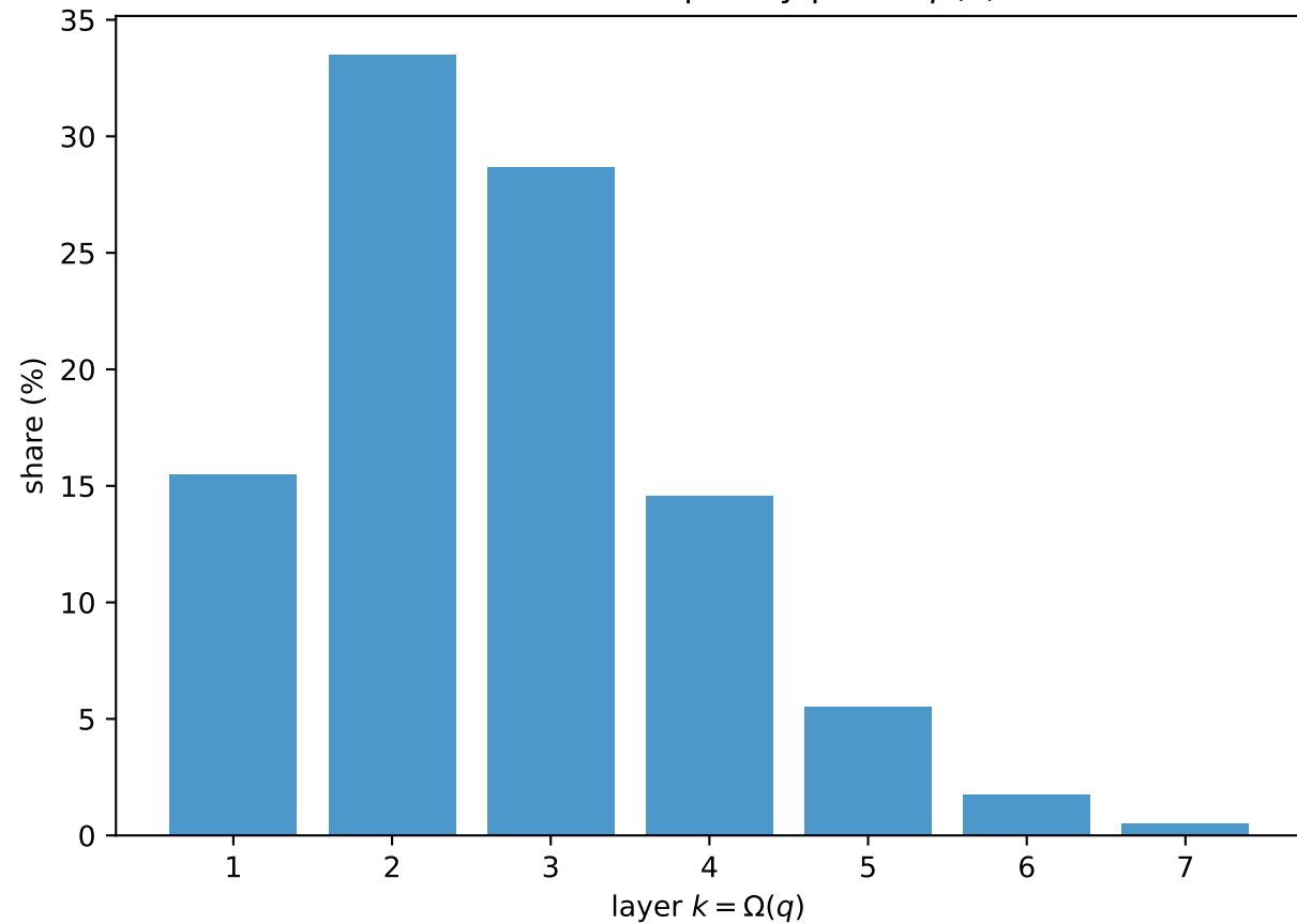
Arithmetic-complexity profile \rho(k)
