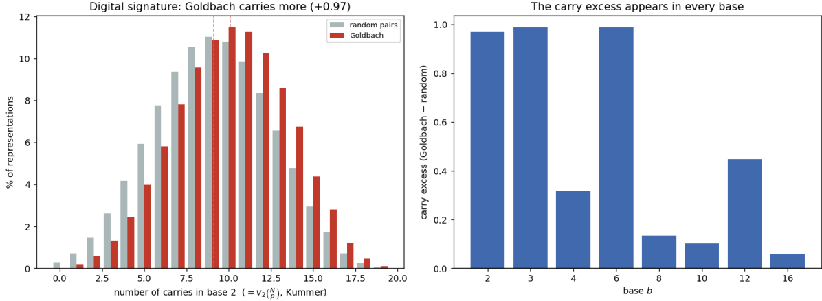
Figure 8: Carry geometry. Left: the distribution of binary carries v_2(\frac{N}{p}) for Goldbach representations (red) versus random pairs (grey)—Goldbach is shifted to more carries (+0.97). Right: the carry excess is positive in every base.
