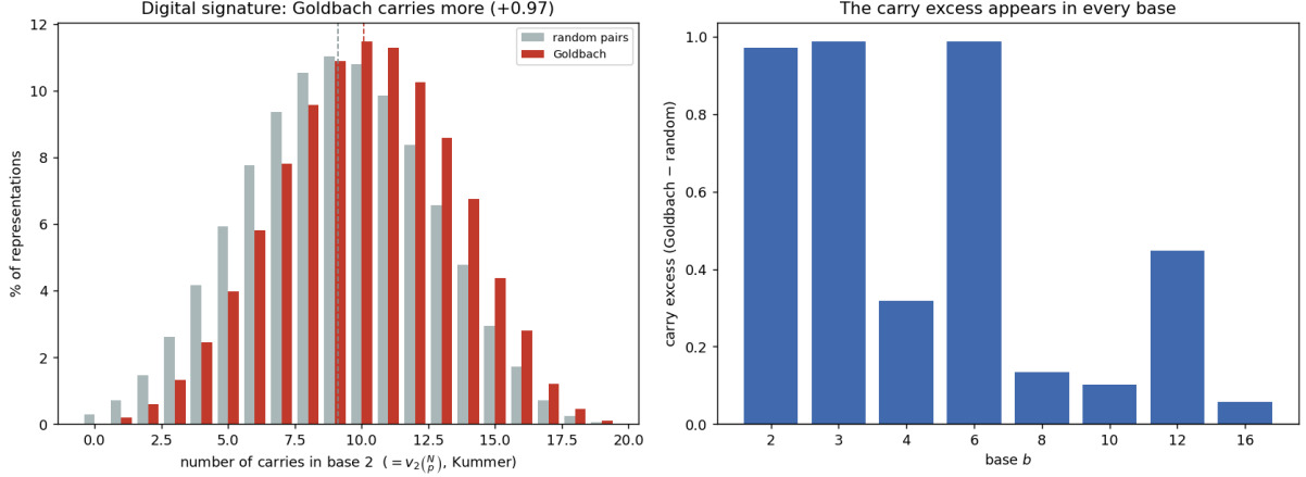
Figure 14: Carry geometry. Left: the distribution of binary carries v_2(N/p) for Goldbach representations (red) versus random pairs (grey)—Goldbach is shifted to more carries ( +0.97 ). Right: the carry excess is positive in every base.
