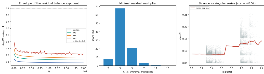
Figure 6. Left: percentile envelope of \lambda_{\text{Res}} = a_{\text{Res}} - 1 versus N , far below the Li–Liu line 0.9. Centre: the minimal multiplier r_{\star} ( r = 3 dominates). Right: \lambda_{\text{Res}} rises with the Goldbach singular series \mathfrak{S}(N) (positive correlation).
