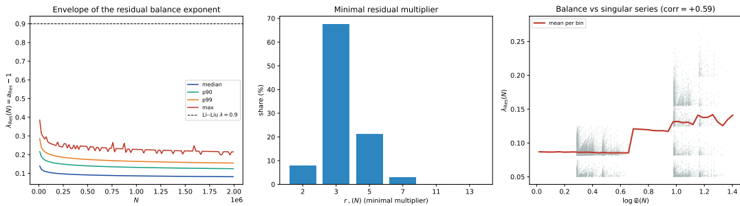
Figure 6. Left: percentile envelope of \lambda_{\text{Res}} = a_{\text{Res}} - 1 versus N , far below the Li–Liu line 0.9. Centre: the minimal multiplier r_{\star} ( r = 3 dominates). Right: \lambda_{\text{Res}} rises with the Goldbach singular series \mathfrak{S}(N) (positive correlation).
