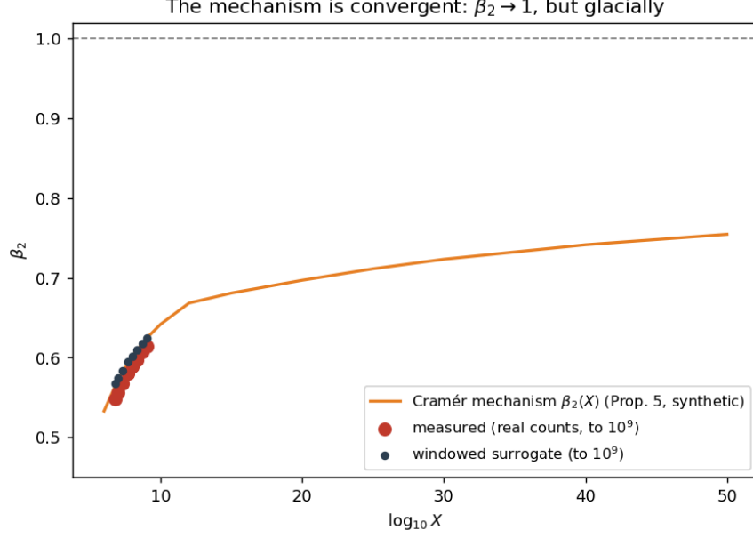
Figure C1. The Cramér mechanism’s effective exponent \beta_2(X) (Proposition 5; synthetic divisibility model), climbing monotonically toward 1 and reaching only \approx 0.75 at 10^{50} , with no plateau. The measured \beta_2 from the real counts (to 10^9 ) lies on the initial segment, and the windowed surrogate agrees. The approach is genuine but glacial ( 1/\log \log X ), which is why no finite computation can see the limit.
