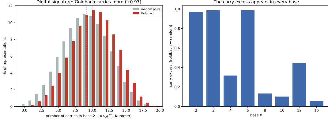
Figure 8. Carry geometry. Left: the distribution of binary carries v_2\left(\frac{N}{p}\right) for Goldbach representations (red) versus random pairs (grey)—Goldbach is shifted to more carries (+0.97). Right: the carry excess is positive in every base.
