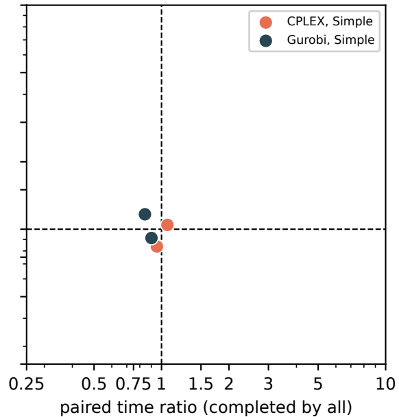
Role-Hybrid vs Base
