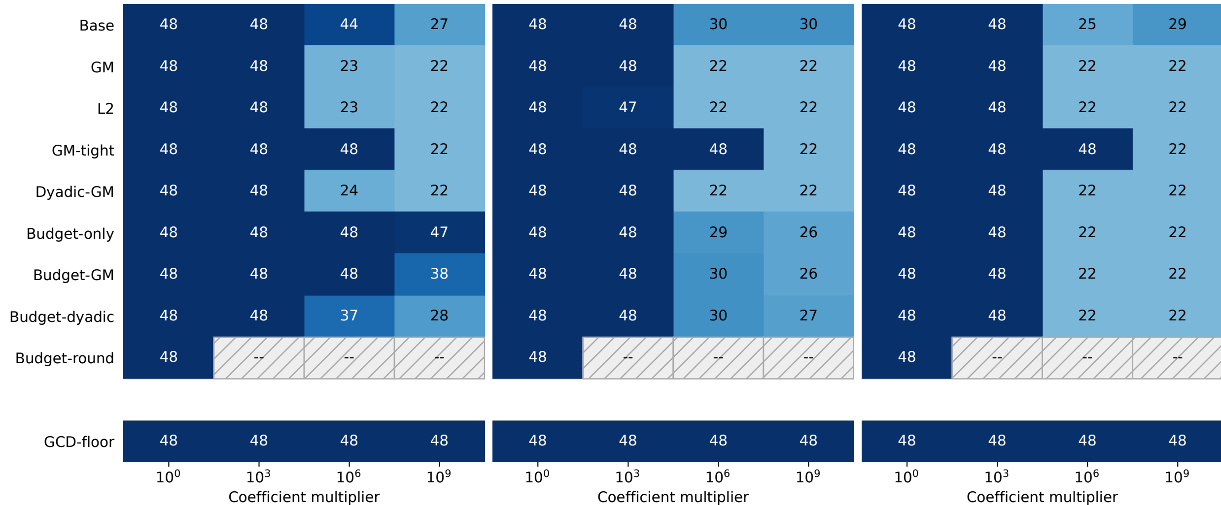
(a) HiGHS 1.15.1
