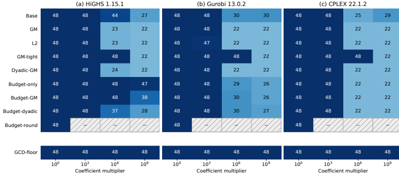
Fig. 2 Verified optima by coefficient multiplier. Each cell counts the configurations whose returned point is a verified optimum, out of the 48 in that cell (three families, eight seeds, two presolve settings). The fixed margin in (7) brings the continuous feasibility boundary increasingly close to an integer activity. Hatched cells marked – are abstentions, where the policy declines to export. The detached bottom row is GCD-floor, the later integer-aware reformulation control, not a scaling policy.
