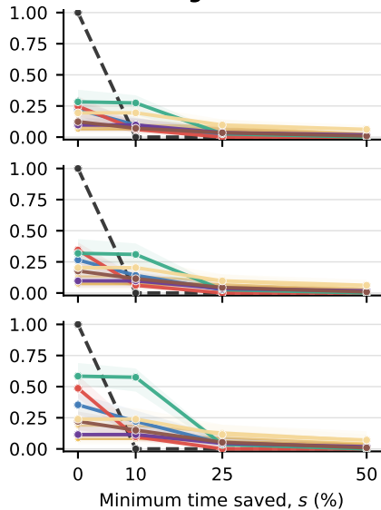
Regression
