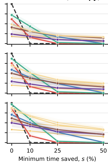
Classification (Entropy)
