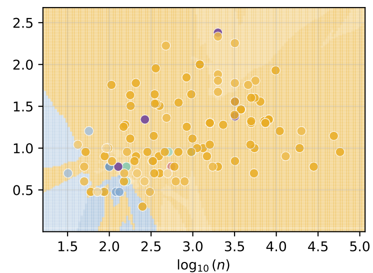
ExtraTree
