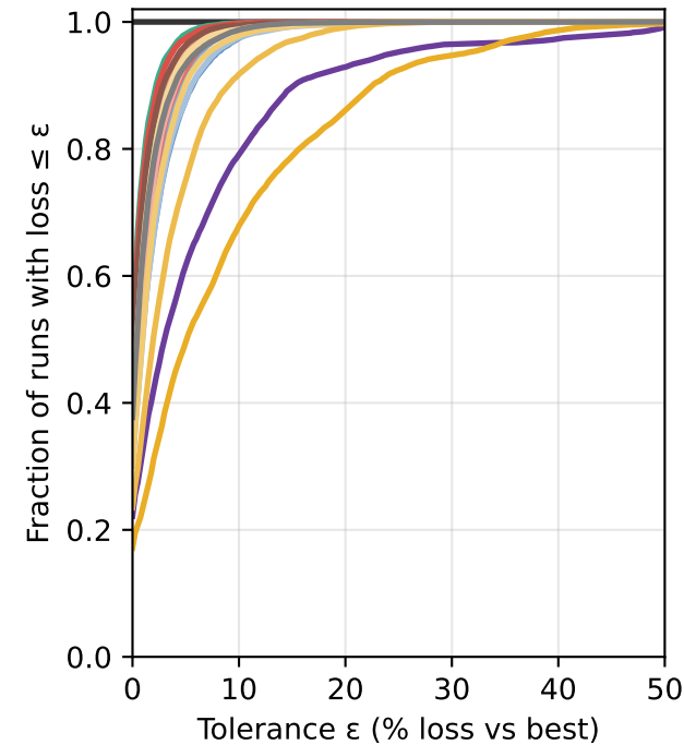
Classification (Entropy) - P(\text{loss} \leq \epsilon) vs \epsilon
