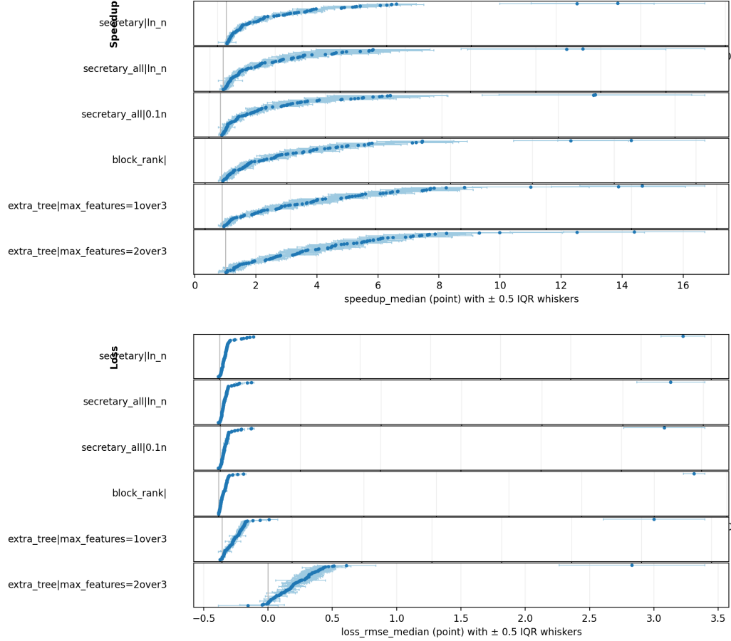
Figure S9: Within-dataset whisker summaries for regression. The upper half of the figure reports dataset-level median speedups for selected methods, and the lower half reports the corresponding dataset-level median RMSE losses. Each point represents one benchmark dataset, ordered within each method panel. Horizontal whiskers indicate \pm 0.5 times the empirical interquartile range over the 50 repeated runs, thereby quantifying within-dataset stochastic variability. The figure makes explicit that methods with similar cross-dataset medians can nevertheless differ substantially in their run-to-run stability.
