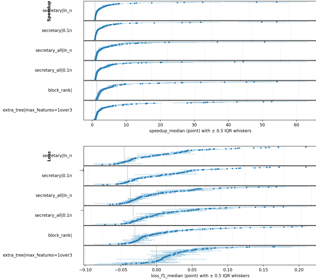
Figure S10: Within-dataset whisker summaries for classification with Gini impurity. As in Supplementary Figure S9, the upper half reports dataset-level median speedups and the lower half reports dataset-level median F1 losses for a selected subset of methods. Each point is one dataset and the whiskers indicate \pm 0.5 times the empirical interquartile range across the 50 repeated runs. The figure shows that several methods achieve similar speedups but differ materially in the stability of their classification loss.
