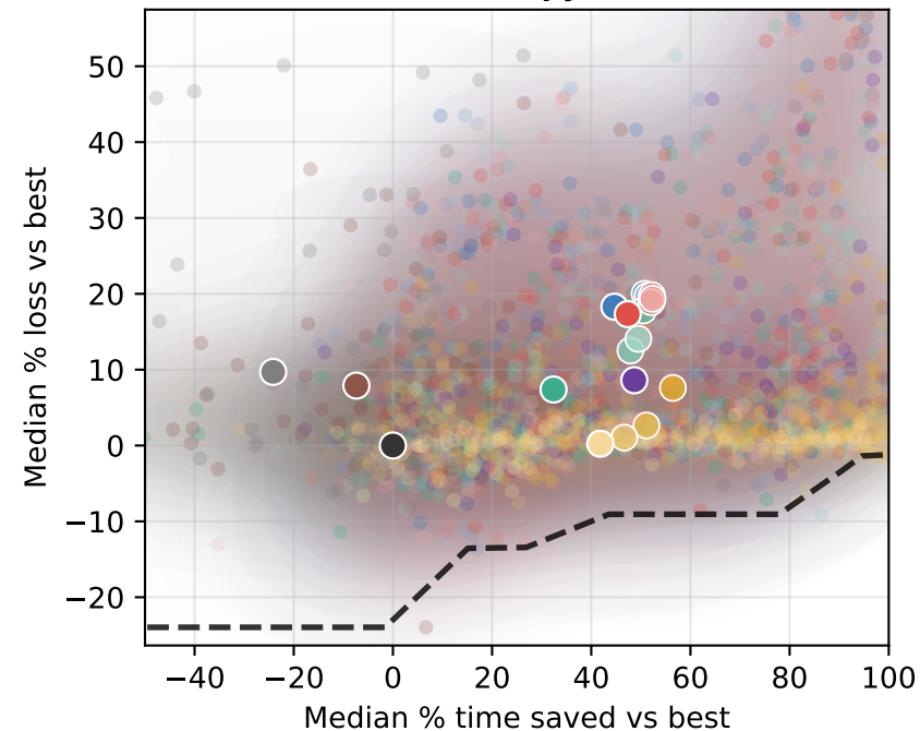
Entropy
