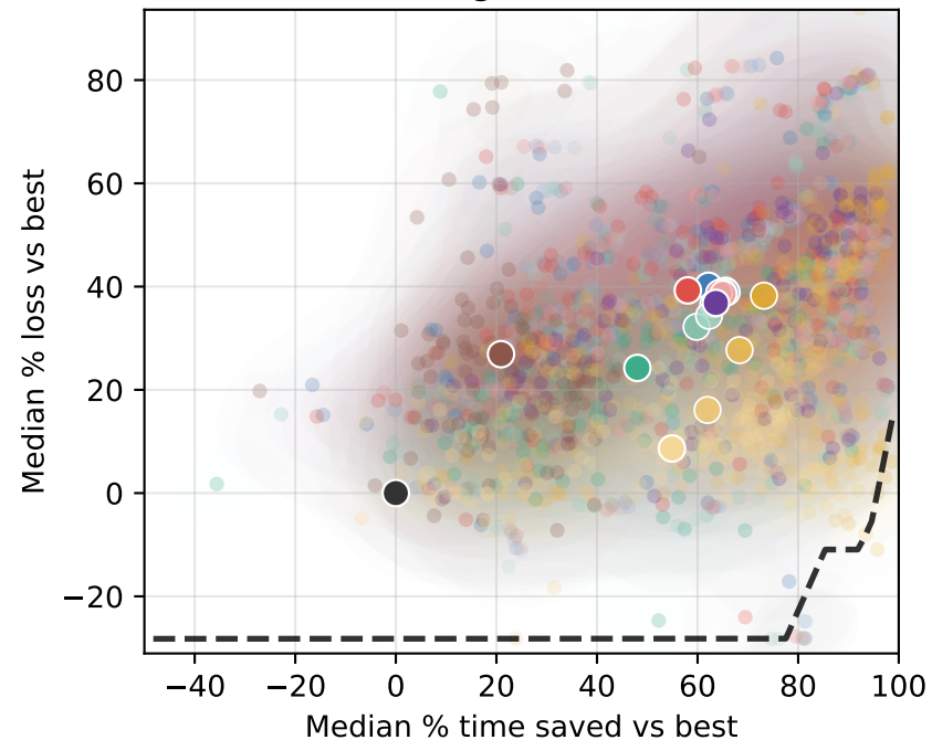
Regression
