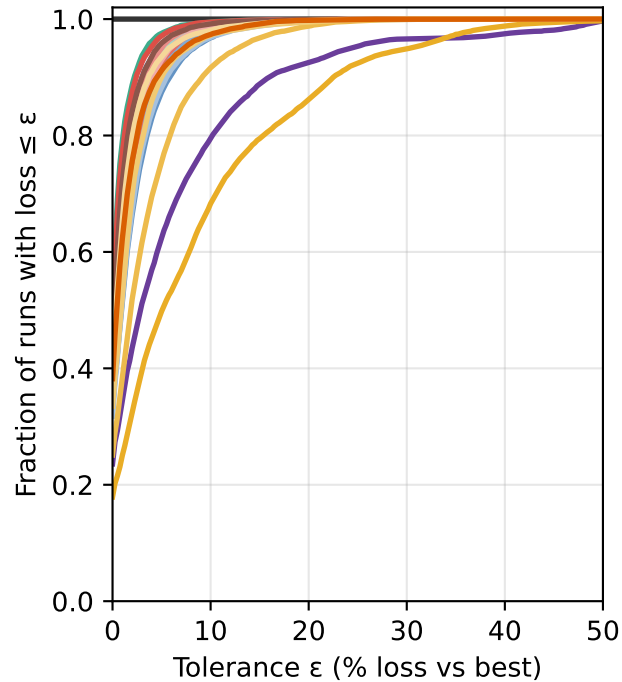
Classification (Gini) - P(\text{loss} \leq \epsilon) vs \epsilon
