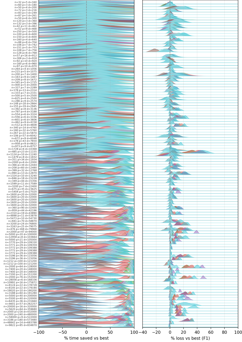
Figure S4: Ridgeline summaries for classification with Gini impurity. Each horizontal ridge corresponds to one benchmark dataset. The left panel shows the empirical distribution, over 100 runs, of the percentage of training time saved relative to the exhaustive splitter, and the right panel shows the corresponding distribution of percentage F1 loss relative to the same baseline. Colors identify methods, and the dashed vertical line at zero marks parity with the exhaustive splitter. Compared with regression, these ridgelines show a much larger concentration of runs near zero predictive loss, which helps explain why secretory-style stopping is more successful in classification.
