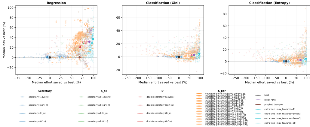
Figure S13: Effort–loss comparison by task. Each point represents one method variant summarized by the median over benchmark datasets. The horizontal axis reports the median percentage of gain evaluations saved relative to the exhaustive splitter, and the vertical axis reports the corresponding median predictive loss. Separate panels are shown for regression, classification with Gini impurity, and classification with entropy impurity. This figure complements the wall-clock Pareto plots by showing how closely time savings track the underlying reduction in exact split-gain computations.
