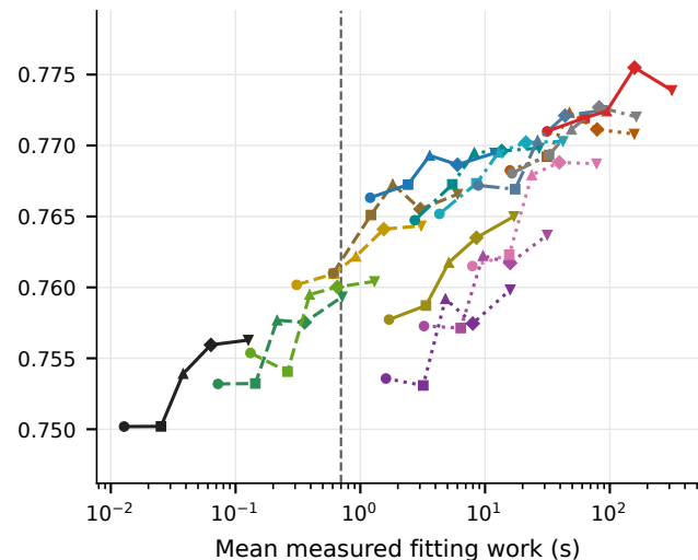
(b) Accuracy versus fitting work
