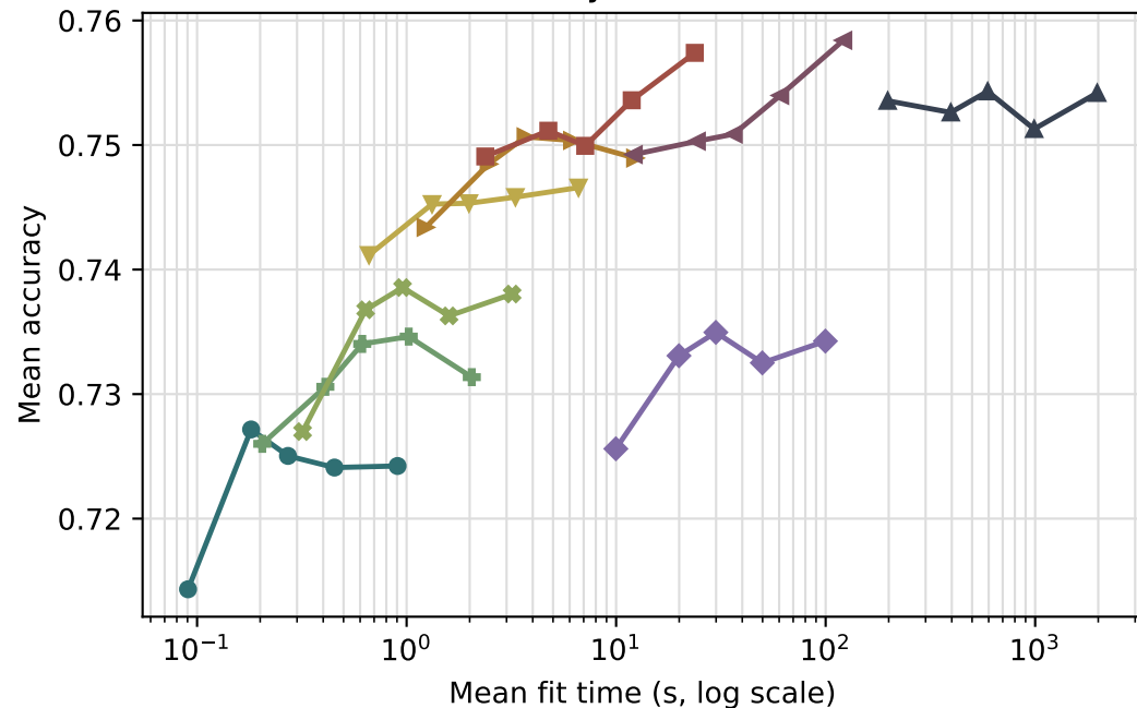
Accuracy-time frontier
