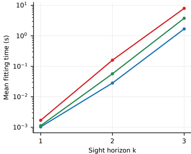
(b) Single-tree fitting cost
