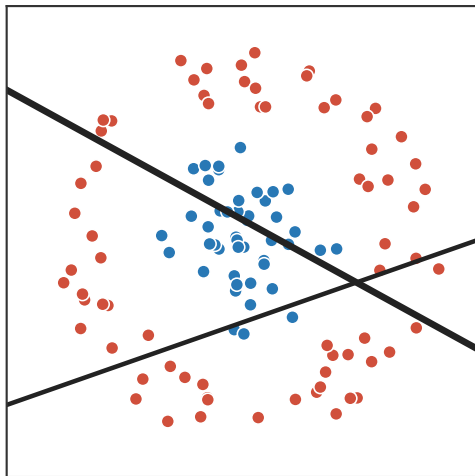
Oblique halfspaces
