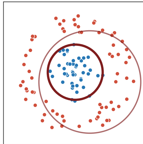
Spherical inside/outside
