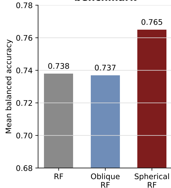
Classification benchmark
