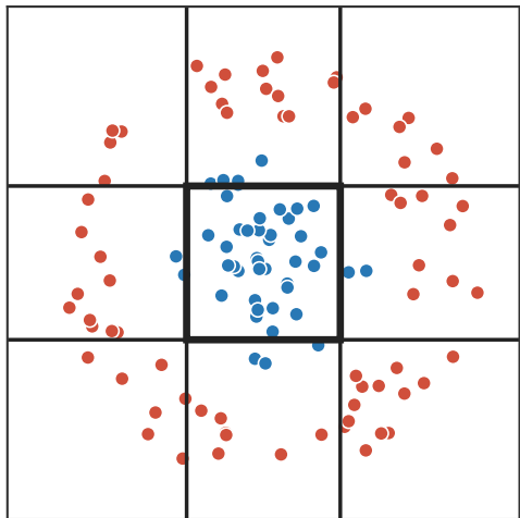
Axis-aligned rectangles
