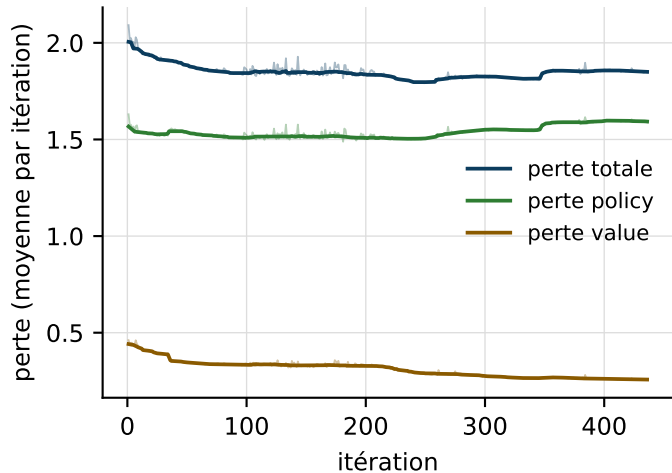
Pertes du self-play
