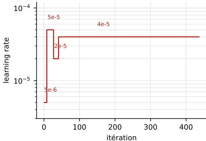
Learning rate (AdamW)
