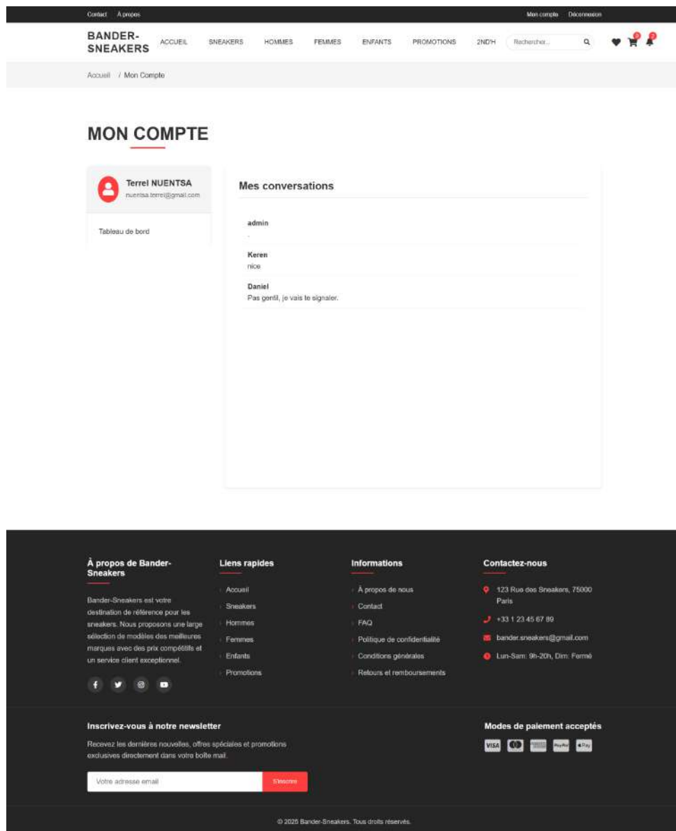
FIGURE 5.19 – Vue conversation
