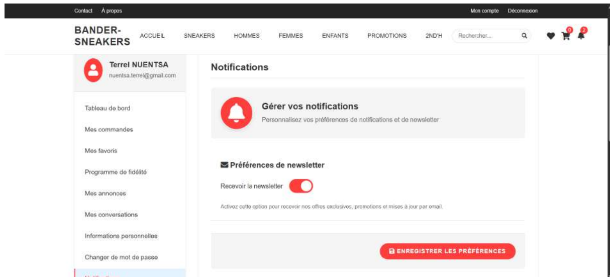
FIGURE 5.34 – Activation/désactivation newsletter
