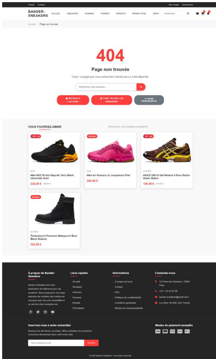
FIGURE 5.37 – Page 404
