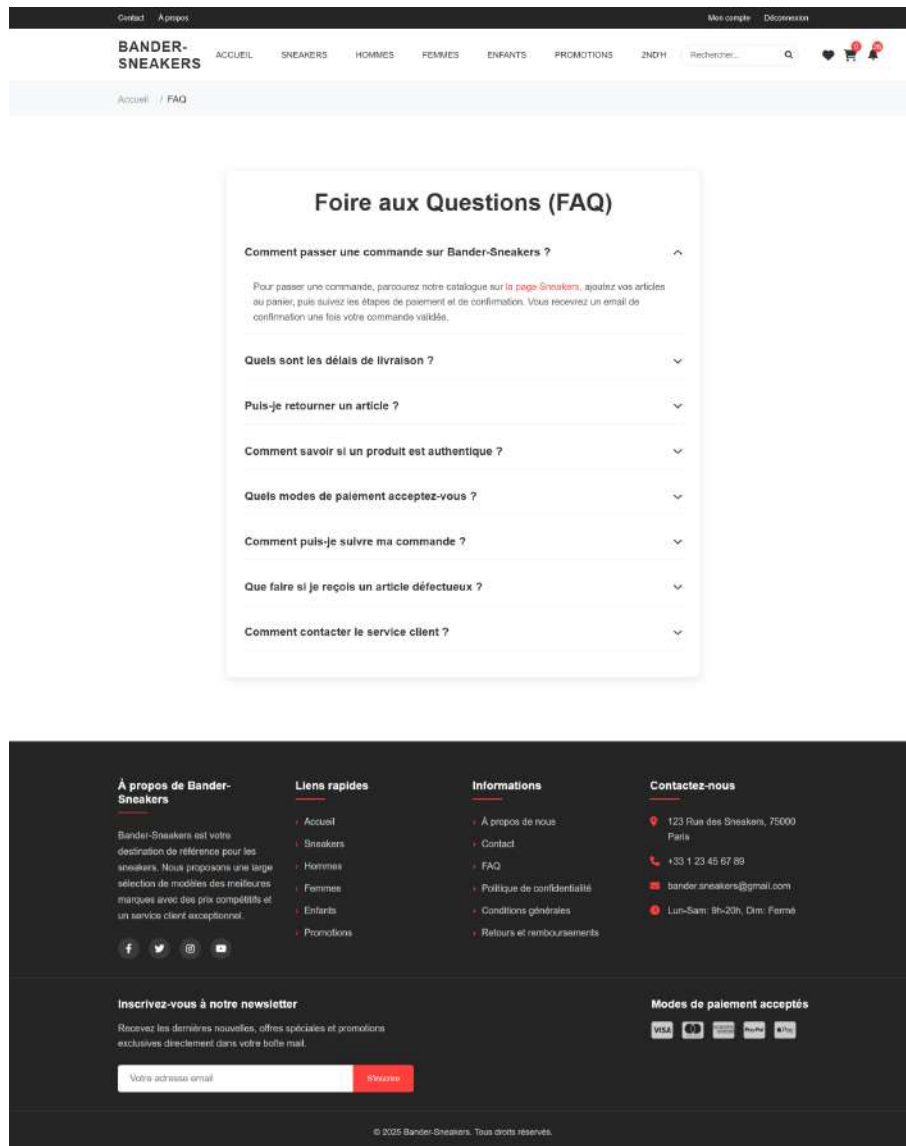
FIGURE 5.42 – Page FAQ
