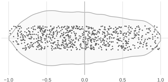
Correlation of all genes to ribosomal genes
