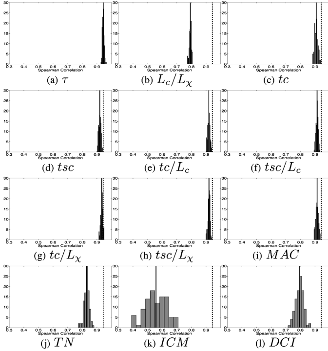
Fig. 12. Histograms of the Spearman correlation values for the various tortuosity measurements on the set of arteries obtained by corrupting with noise the manually traced vessel center points. In each panel, the solid vertical line is the median value of the histogram, and the dashed vertical line is the median of the values of the proposed tortuosity \tau , shown for comparison.
