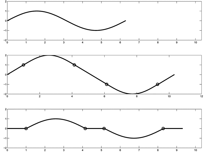
Fig. 3. Three curves with the same curvature but different aspect. In the top panel, a sinusoid is shown, and in the middle and bottom panel the same sinusoid is split in half with the two parts linked by straight lines. Circles show the limits of the two sinusoid halves.
