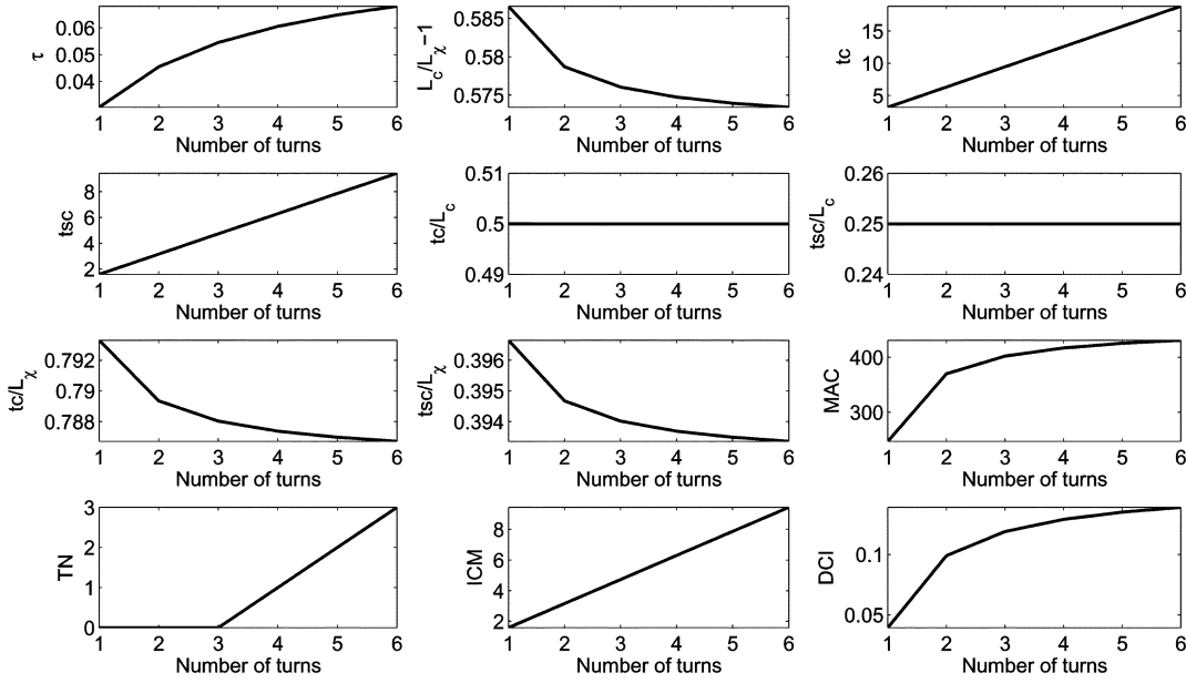
Fig. 11. Tortuosity indexes as a function of the number of the composing circular arcs, for the third simulated vessels set.
