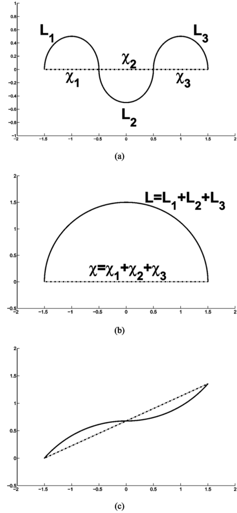
Fig. 2. First two curves [(a) and (b)] have very different tortuosity but the same arc length L and chord length \chi . Second and last curves [(b) and (c)] have the same mean angular difference (MAC) despite their different perceived tortuosity. Curve in (c) has a curvature integral of \pi/2 , whereas the one in (b) has curvature integral \pi , even if the one (c) is perceived as more tortuous.
