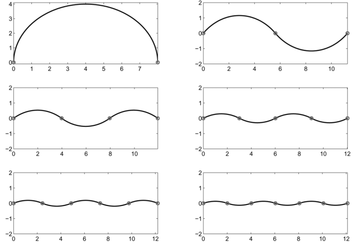
Fig. 4. Simulated vessels obtained by breaking a semi-circular arc into smaller arcs, and arranging them so that each arc has curvature sign different from the preceding one. The circles represent the points of changing curvature sign.
