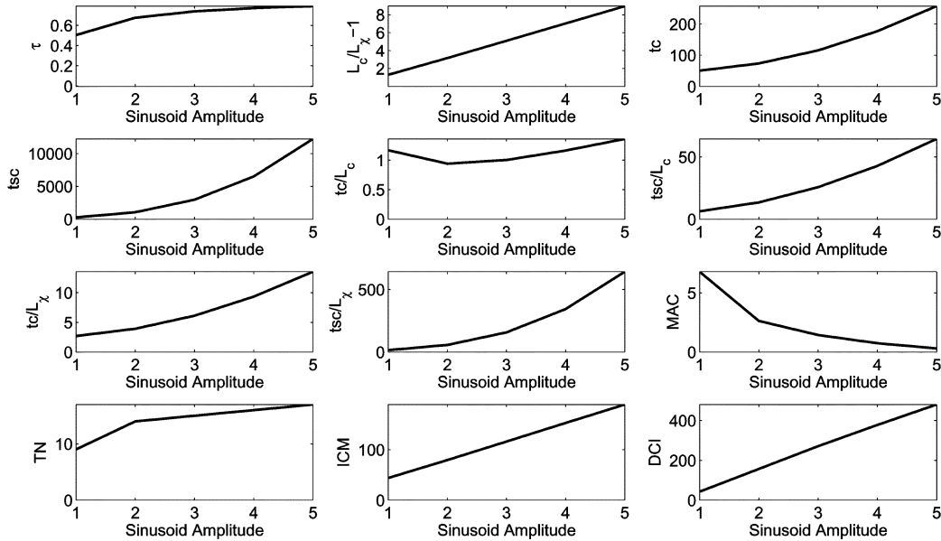
Fig. 10. Tortuosity indexes as a function of the amplitude, for the second simulated vessels set.
