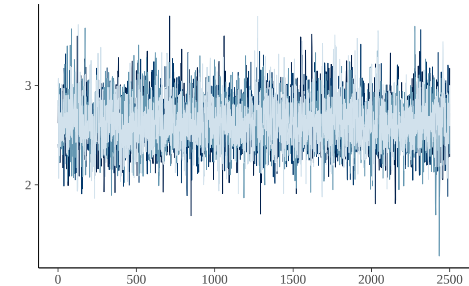
b_dprime_Intercept
