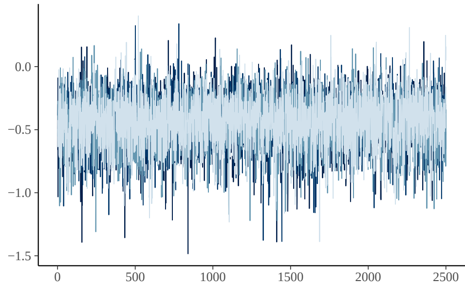
b_Intercept
