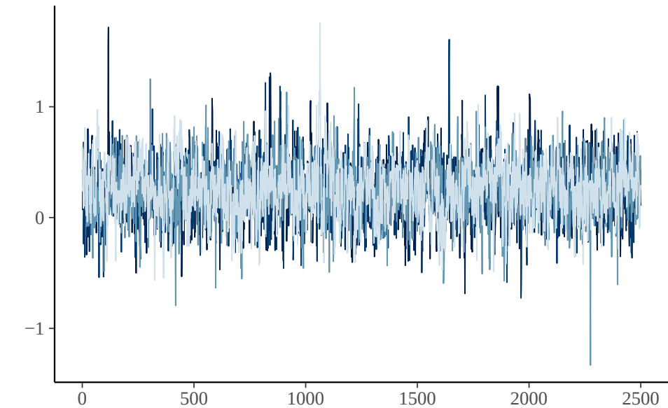
b_c_Intercept
