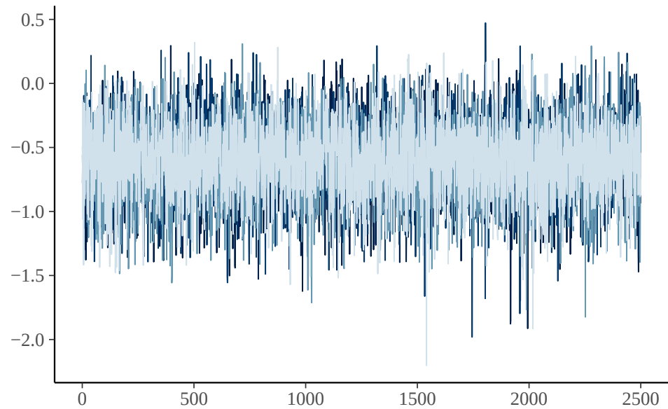
b_contextFission
